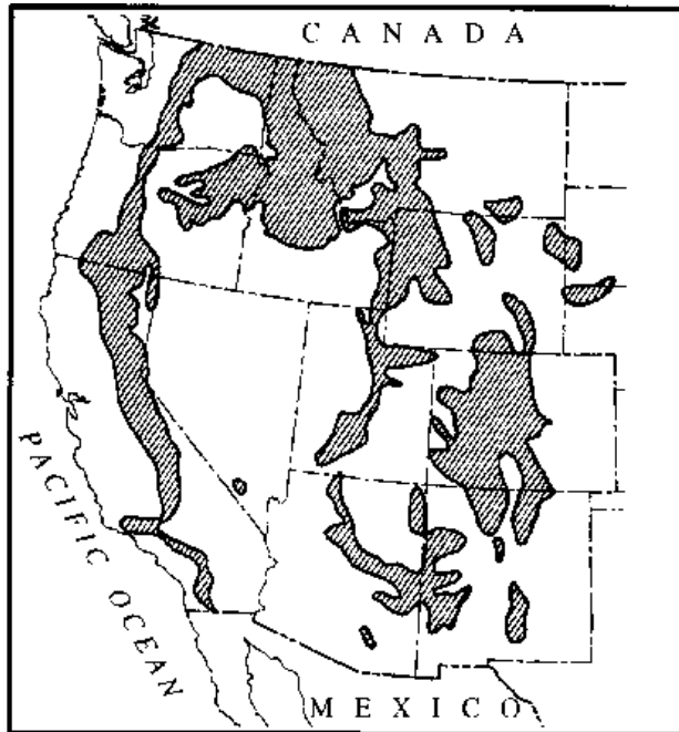
Figure 1. Distribution of Ips pini in the western United States
