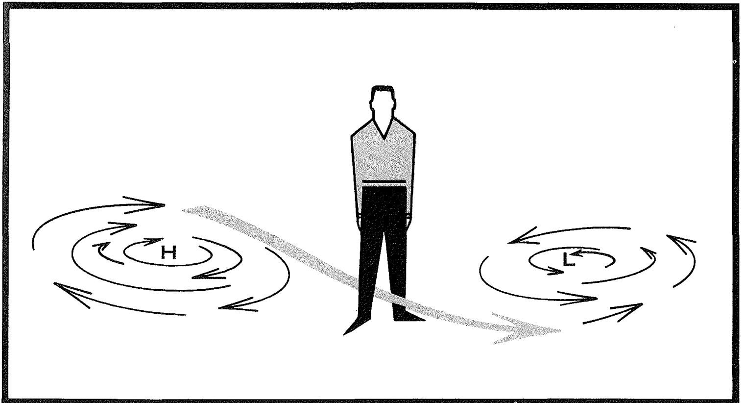
"Back to the wind, high pressure on the right" is a useful rule. Because of friction, air near the surface flows from high- to low-pressure areas. Air accumulated near the surface in Low centers is forced aloft; the removal of air from High centers requires downward displacement of air.
