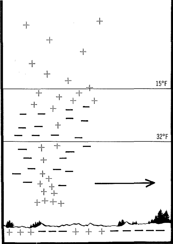
As a thunderstorm cloud becomes electrified, positive charges tend to accumulate in the top of the cloud and negative charges in the lower portion. Smaller positive and negative charge areas also develop. Rapidly falling rain carries positive charges downward and creates a positive charge center in the precipitation core.
