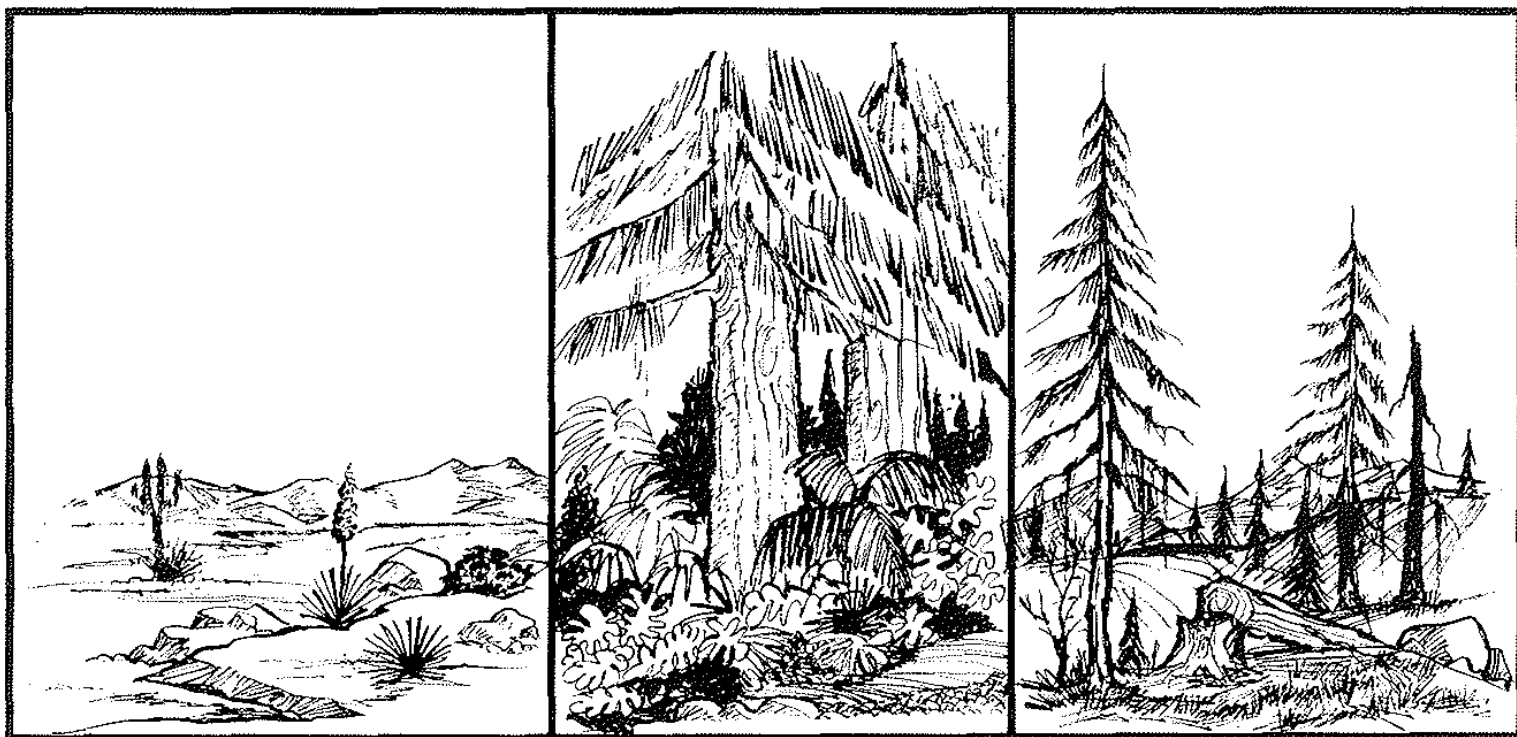
Where vegetation is plentiful, fire potential depends largely upon moisture content. The rain forest may be fire-safe virtually all the time, while the parched forest at times may be explosive.
