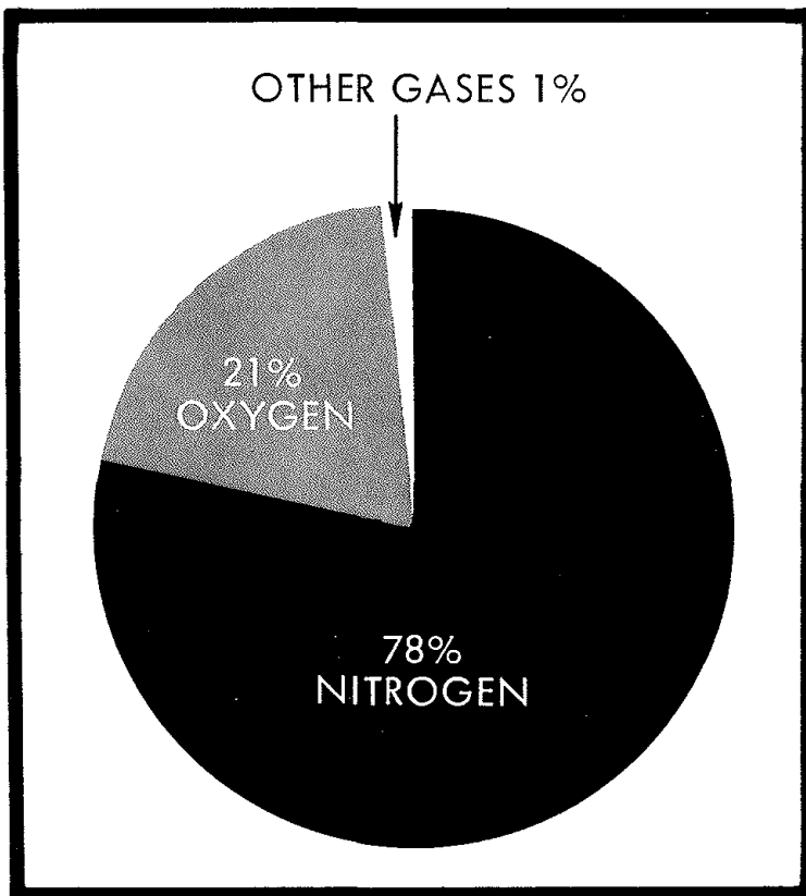
Air in the troposphere is composed mostly of two gases—nitrogen and oxygen.
