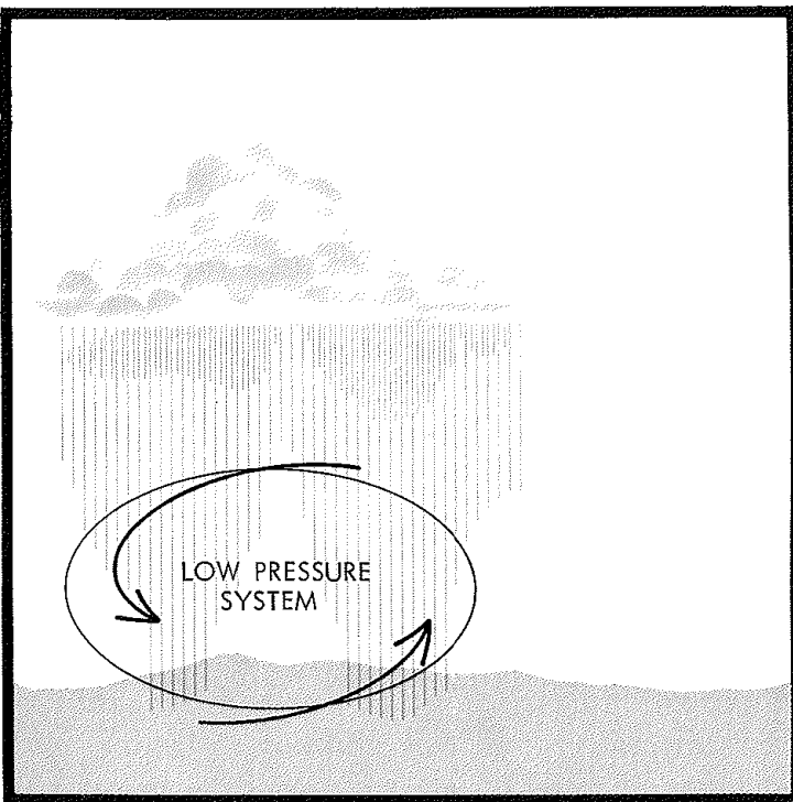
Air around a Low flows counterclockwise in the Northern Hemisphere and spirals inward. This converging airflow produces rising motion, and, if sufficient moisture is present, precipitation will result.
