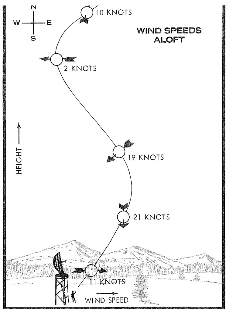
Wind speeds and directions aloft in a stratified atmosphere may vary from one layer to the next. The arrows indicate horizontal directions according to the compass card in the upper left.
