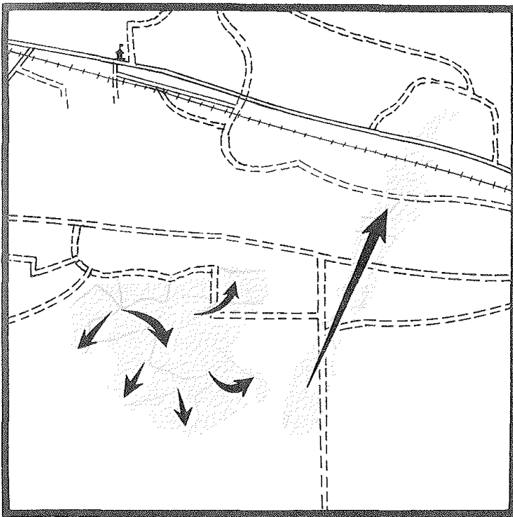
The nature of the wind during a wildfire is shown by the shape of the burned area. Turbulent winds usually cause more erratic fire behavior and firespread in many directions, while laminar flow is likely to result in spread in one direction.
