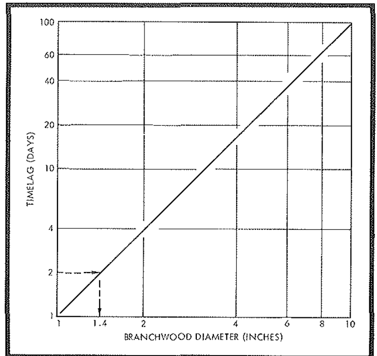
The average timelag period of branchwood and logs varies with the fuel diameter. Other fuels may be compared with these. A 2-inch litter bed with an average timelag period of 2 days, for example, may be considered the equivalent of 1.4-inch dead branchwood having the same average timelag period.
