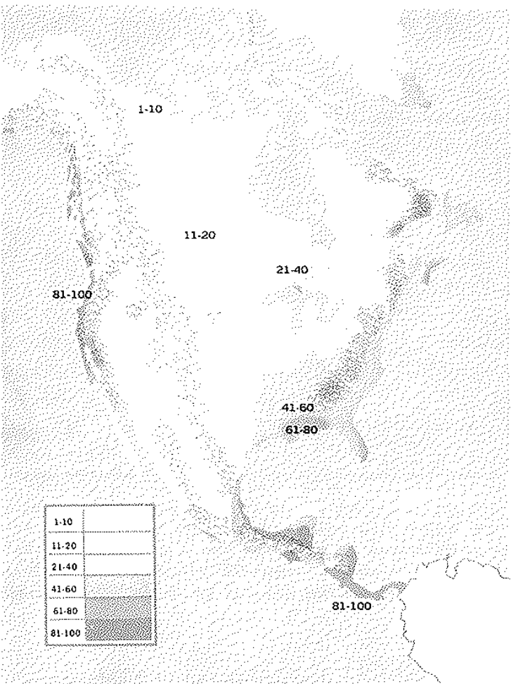
Annual precipitation varies widely over North America. Maximum precipitation is along the Pacific Northwest coast and the Gulf coast. Lowest amounts occur in the Great Basin, the Southwest semidesert and desert regions, and the Arctic region.
