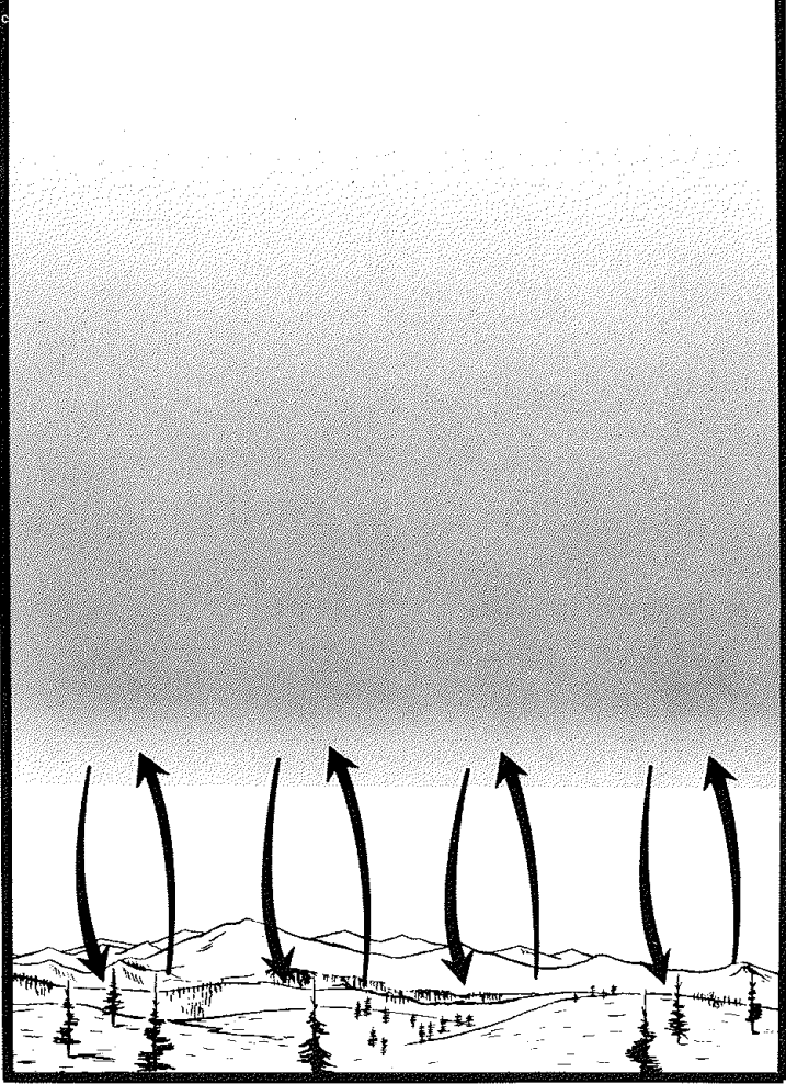
Daytime convective currents may eat away the base of a subsidence inversion and mix some of the dry air above with the more humid air below. This process will warm and dry the surface layer slightly, but humidities cannot reach extremely low values unless the subsiding air reaches the surface.
