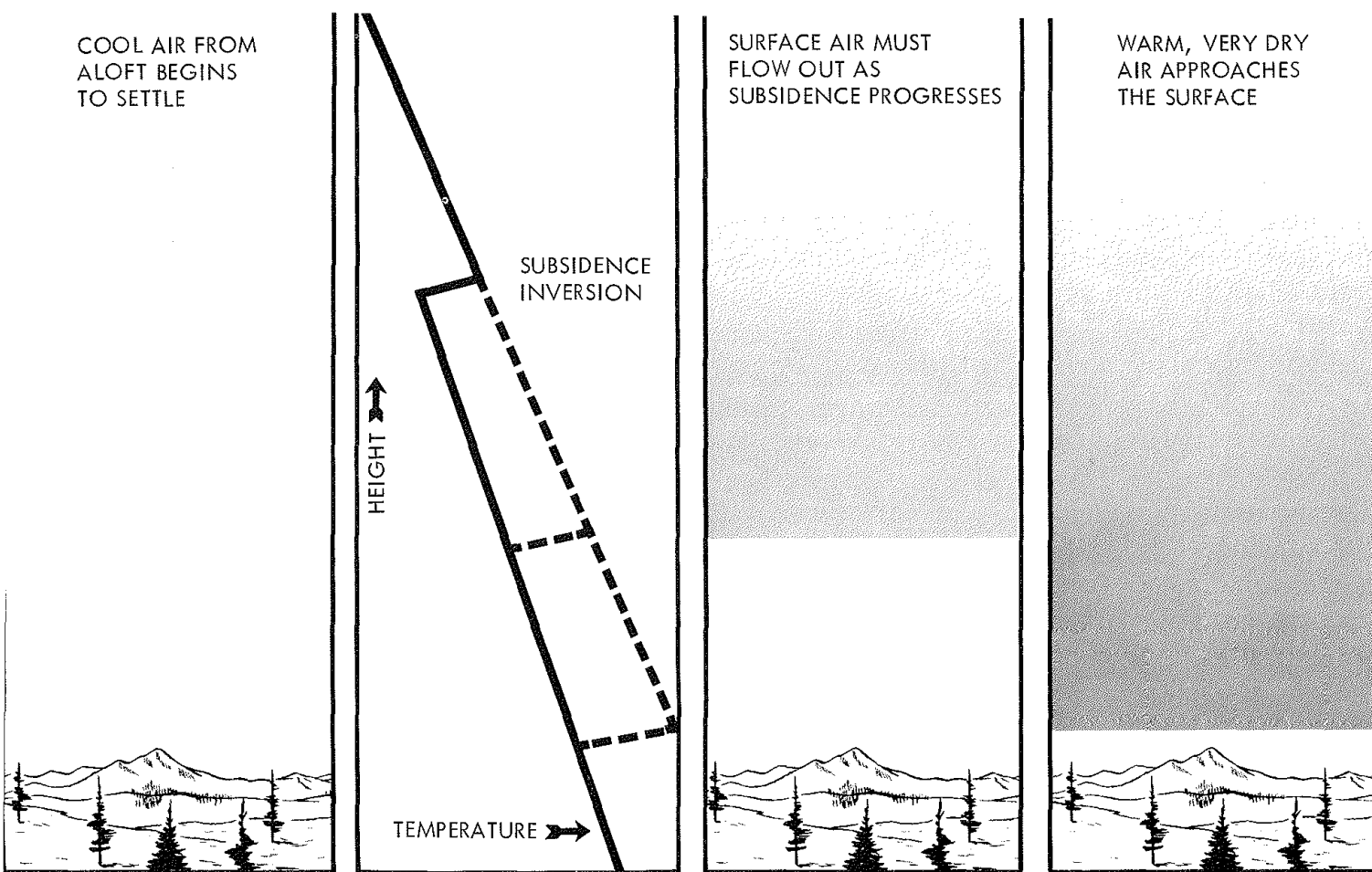
The descent of a subsidence inversion may be followed on successive soundings, as shown by dashed lines. As the more humid surface air flows outward, the drier air aloft is allowed to sink and warm adiabatically.
