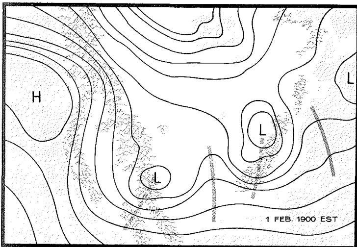
These two 500 mb. charts, 12 hours apart, illustrate short waves moving through the long-wave pattern. Short waves are indistinct in the long-wave ridge position in the Gulf of Alaska. Short-wave troughs, shown by dashed lines, tend to deepen in the long-wave trough position which extends into Northern Mexico. Short-wave ridges, shown by solid lines, are indistinct in the long-wave trough, but develop as they move out of the trough, as did the one which moved from the Southwest and Northern Mexico into the Mississippi Valley.
