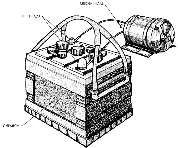
Chemical energy can be transformed into electrical energy, which in turn can be transformed into mechanical energy or thermal energy.
