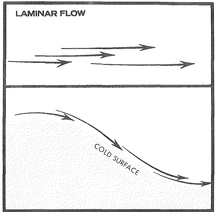
In laminar flow there is little mixing. The air flows smoothly along, one layer seeming to slide over the next. Laminar flow is characteristic of cold air flowing down an incline.
