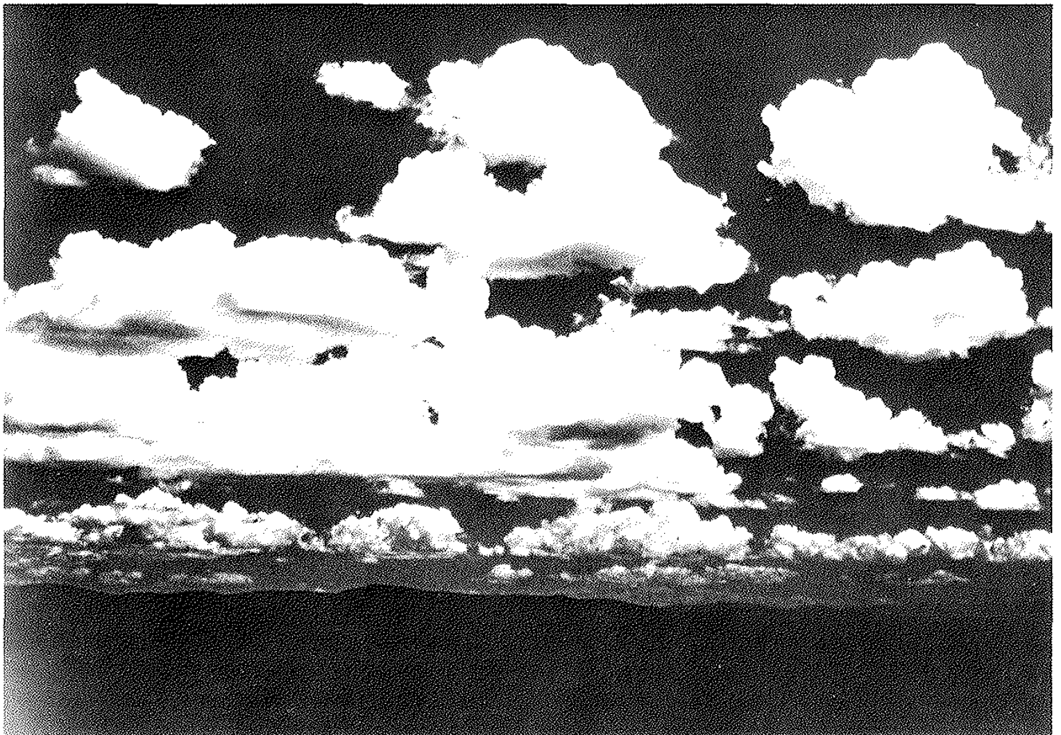
Cumulus clouds are detached clouds in the form of rising mounds or domes. They are dense, have sharp outlines, and the upper portion often resembles a cauliflower. They are composed of a great density of small water droplets; ice crystals may appear in the tops of larger cumulus.
