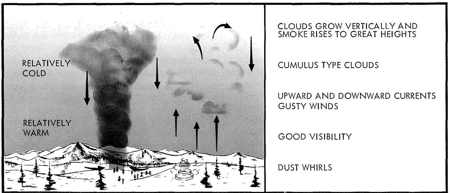
Visible indicators of an unstable atmosphere.
