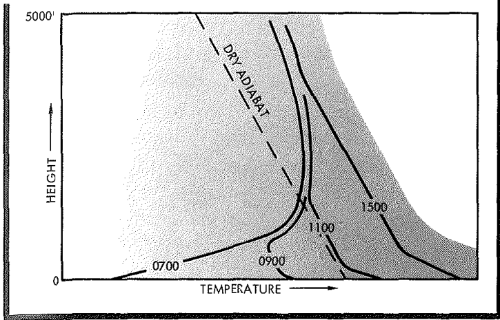
A night surface inversion (0700) is gradually eliminated by surface heating during the forenoon of a typical clear summer day. A surface superadiabatic layer and a dry-adiabatic layer above deepen until they reach their maximum depth about midafternoon (1500).
