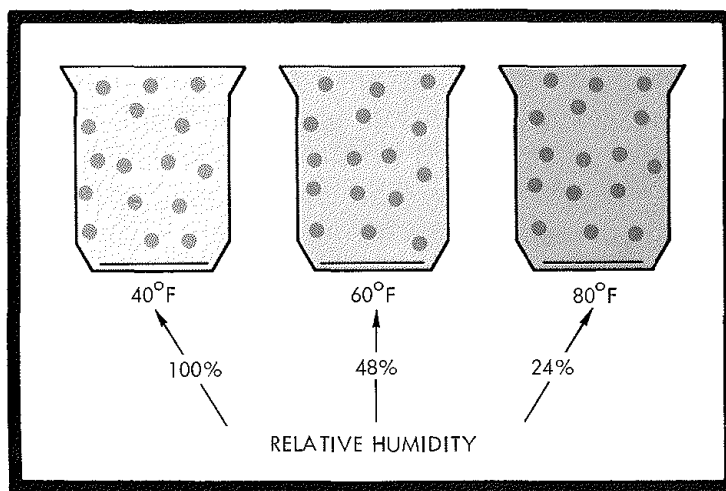
Relative humidity decreases as temperature increases even though the amount of water vapor in the air remains the same.
