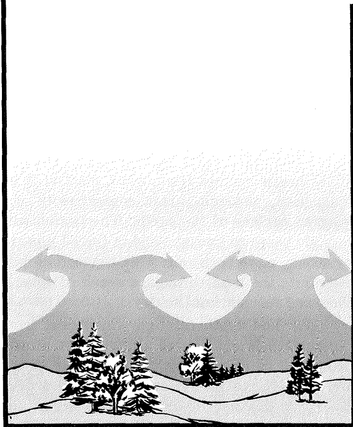
In a stable air mass, the daytime heating and mixing are confined to a shallow layer, and the temperature of this air will increase rapidly.
