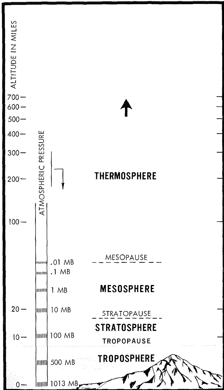
Pressure decreases rapidly with height through the troposphere and stratosphere.
