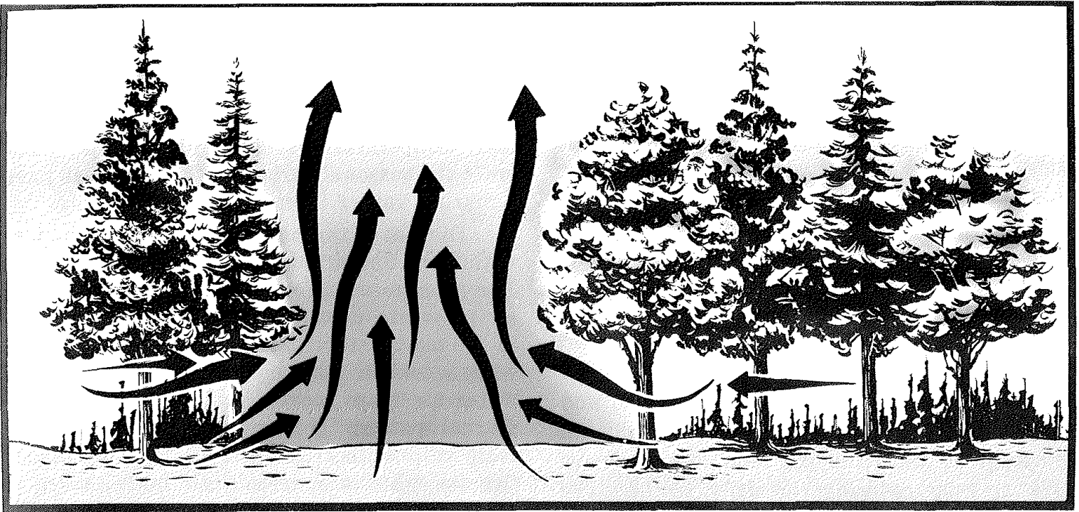
Openings in a timber stand tend to act as chimneys under conditions of strong daytime heating and light winds.
