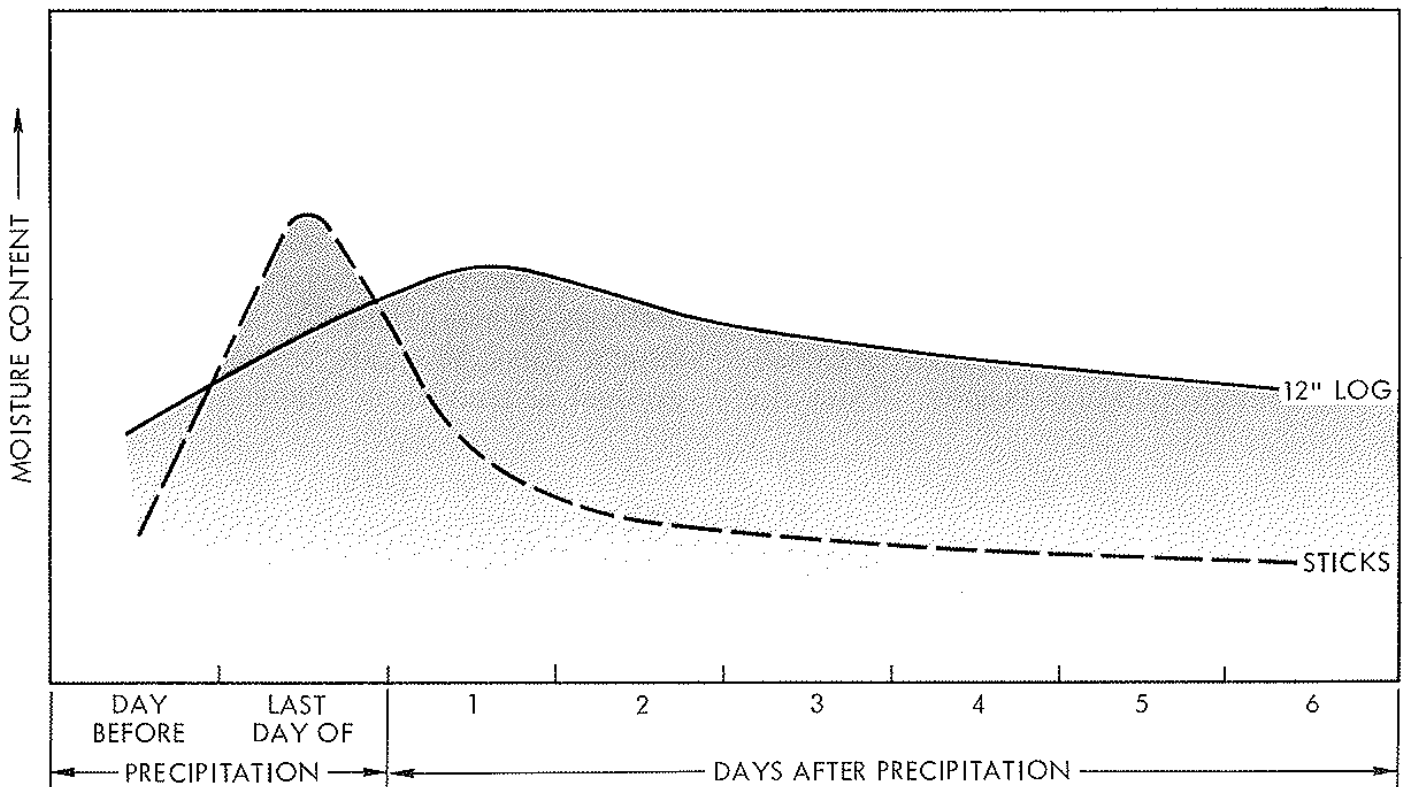
Measurements of the moisture contents of different sizes of fuels before, during, and after precipitation show that larger fuels, such as logs, are slow to react to both wetting and drying.
