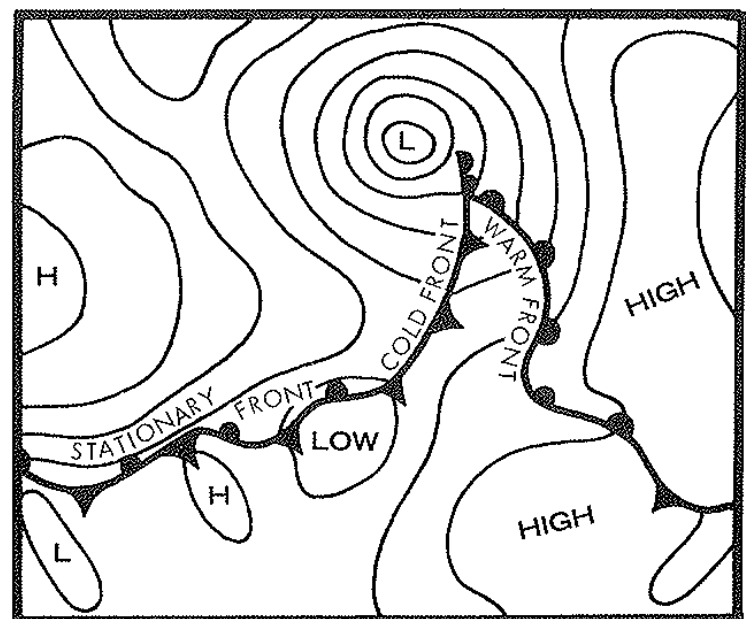
Fronts are classified by the way they move relative to the air masses involved. At a cold front , cold air is replacing warm air. At a warm front , warm air is replacing cold air. A stationary front , as the name implies, is temporarily stalled.
