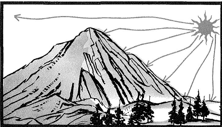
Upper left.—Surfaces more nearly perpendicular to incoming radiation receive more heat per unit area, and become warmer, than do those more nearly parallel to the incoming radiation. Lower left.—As the sun arcs across the sky, its rays are more nearly perpendicular to different slopes and aspects at various
