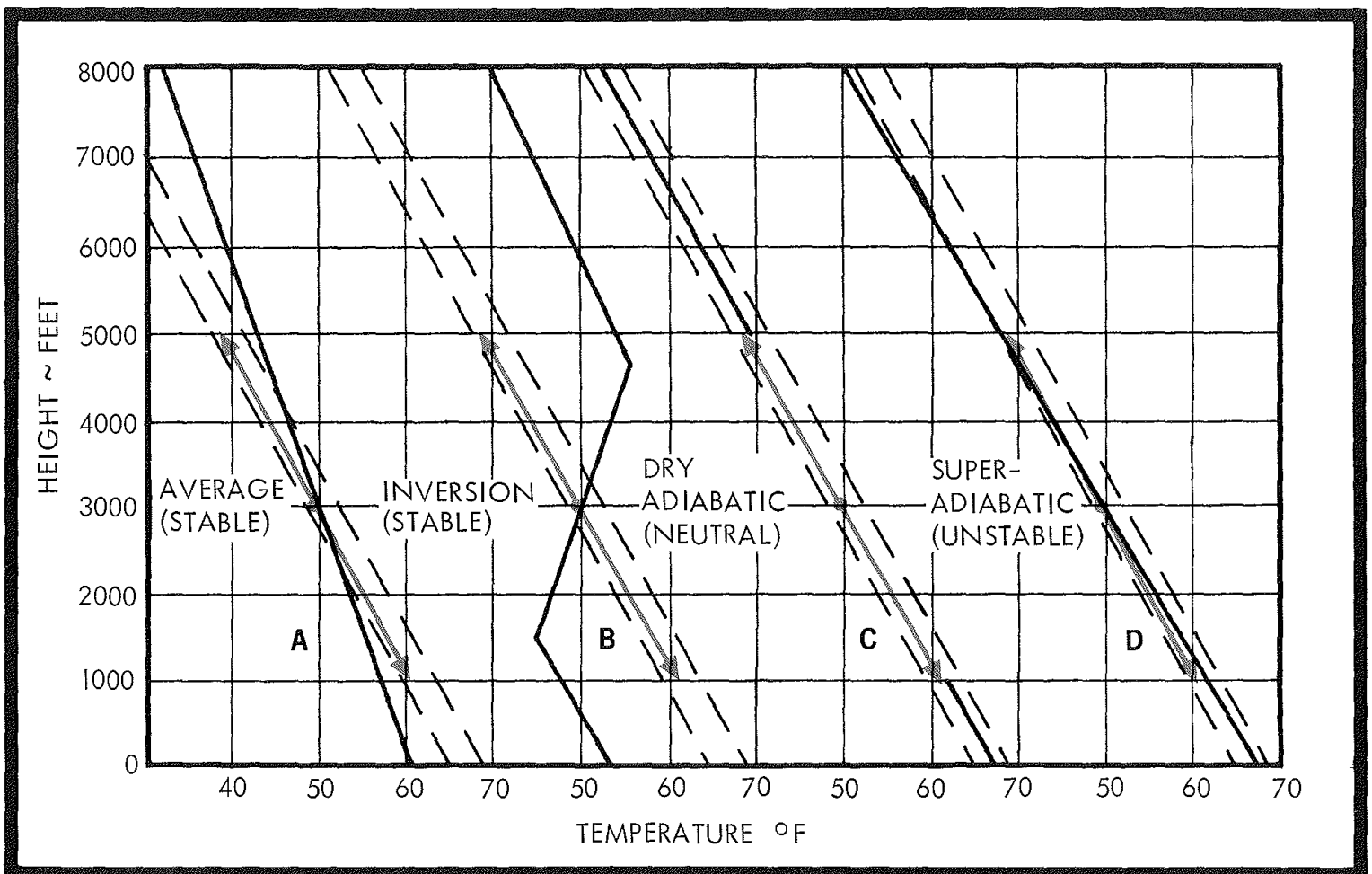
In unsaturated air, the stability can be determined by comparing the measured lapse rate (solid black lines) to the dry-adiabatic lapse rate (dashed black lines). The reaction of a parcel to lifting or lowering may be examined by comparing its temperature (red arrows for parcel initially at 3,000 feet and 50°F.) to the temperature of its environment.
