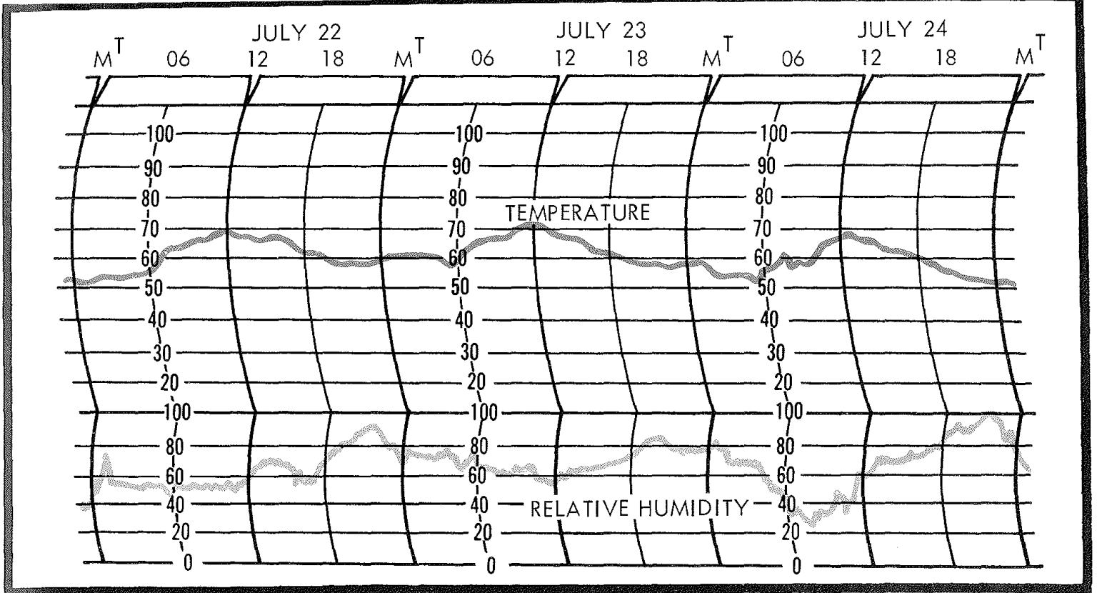
Temperature and relative humidity traces at mountain stations are often less closely related than at valley stations. Changes in absolute humidity are more important at mountain stations.
