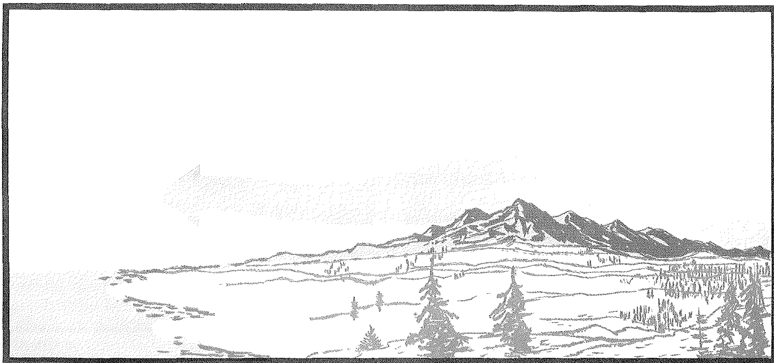
A weak foehn may override cooler air on the lee side of the mountains. In these cases only the higher elevations are affected by the foehn flow.
