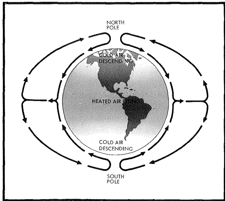
If the general circulation could be represented by a simple convective circulation, heated air at the Equator would rise to near the tropopause, then spread out both north and south. Toward the poles, it would cool, and finally descend and move back to the Equator.
