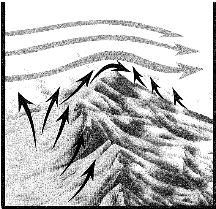
General winds are modified by local wind flow. Weak general winds may exist only at or above ridgetops when strong upslope winds predominate. Upslope winds may establish or intensify wave motion in the general wind flow.
