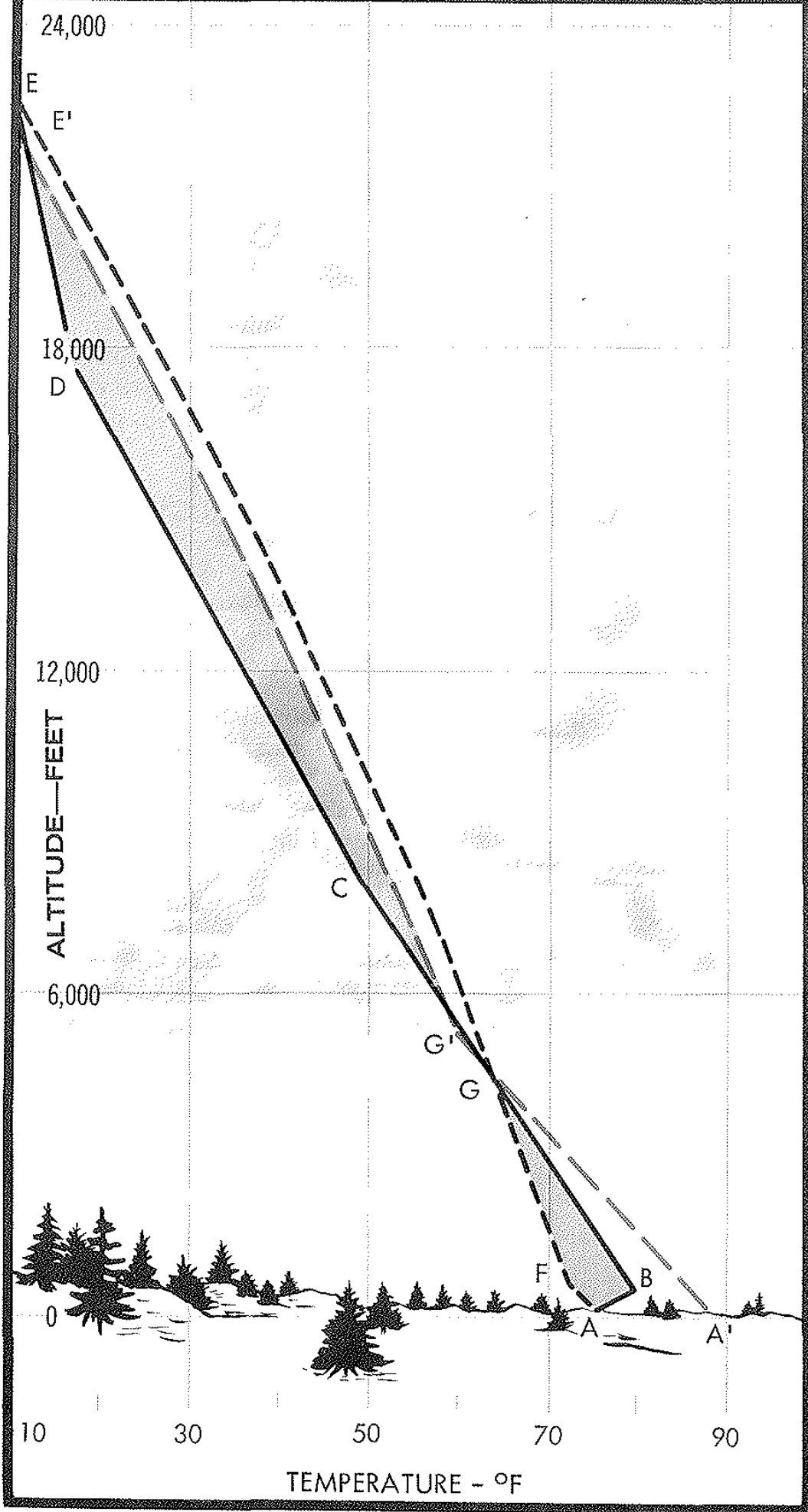
Thunderstorms can be triggered in a conditionally unstable atmosphere by surface heating. Line ABCDE represents an early morning lapse rate, and A'G'CDE a corresponding afternoon lapse rate.
