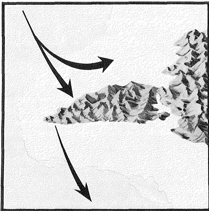
General winds along an irregular or crooked coastline may oppose a sea breeze in one sector and not in another.
