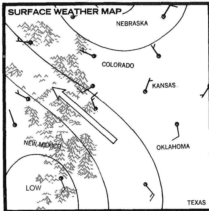
The wind directions at surface stations may differ widely from the windflow above the friction layer, as shown by this weather map. Surface wind direction is indicated on weather maps by a wind arrow flying with the wind. The number of barbs on the tail represent the wind speed. At the top of the friction layer the wind blows parallel to the isobars, as shown by the large arrow.
