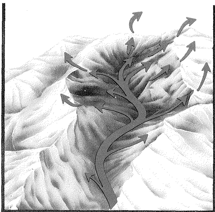
The combined upslope and upvalley winds proceed upstream during the day and continually divide at each tributary into many upravine and upslope components.
