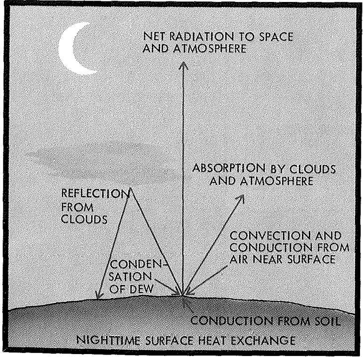
At night there is net cooling of the earth's surface although some heat is returned by various methods.
