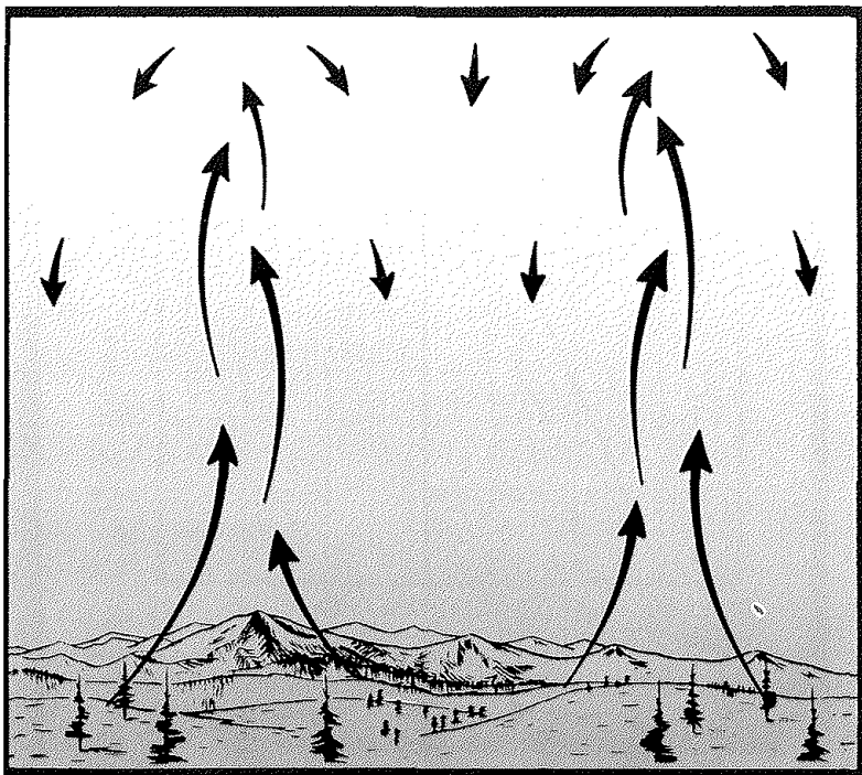
Convection is a process by which air is lifted in the atmosphere. Surface heating during the daytime makes the surface layer of air unstable. After its initial inertia is overcome, the air is forced upward by the more dense surrounding air.
