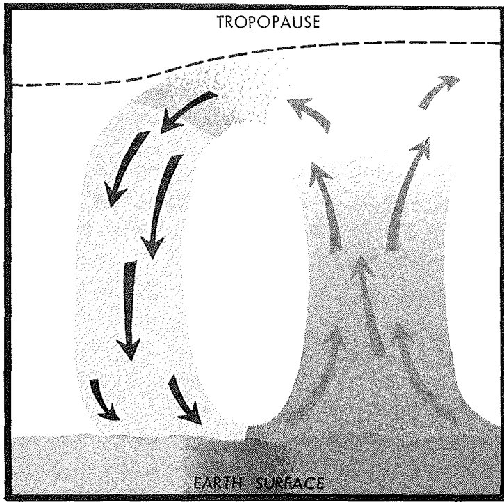
In a simple convective circulation, warm air expands and is forced aloft. As it cools, it descends and returns to the heat source.
