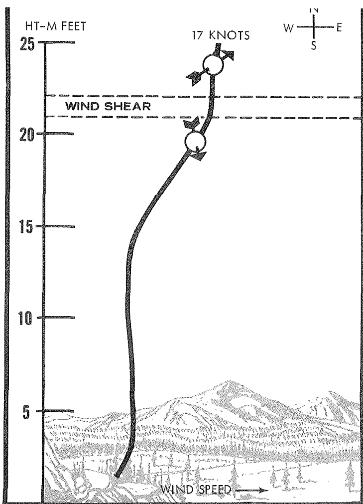
A sharp change in direction also causes wind shear. Shear layers usually indicate that the atmosphere is stratified into layers.
