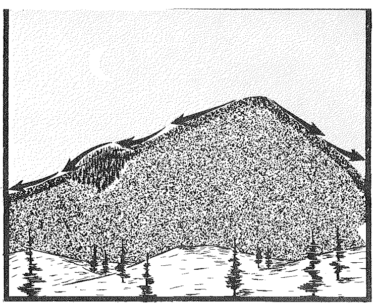
Downslope winds are shallow, and the flow tends to be laminar. The cold air may be dammed by obstructions such as dense brush or timber.
