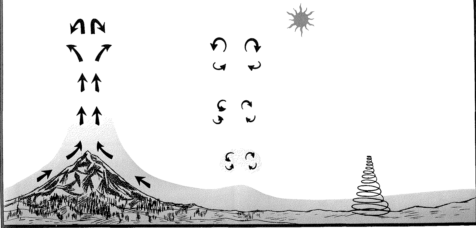
Strong surface heating produces several kinds of convective systems. Upslope winds develop along heated slopes. Superheated air in flat terrain escapes upward in bubbles or in the form of whirlwinds or dust devils.
