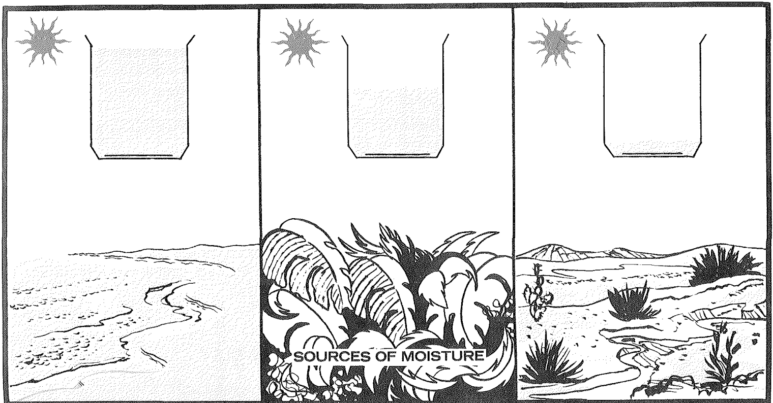
Although the oceans are the principal source of atmospheric moisture, transpiration from plants is also important. But in arid areas, transpiration adds little moisture to the atmosphere.
