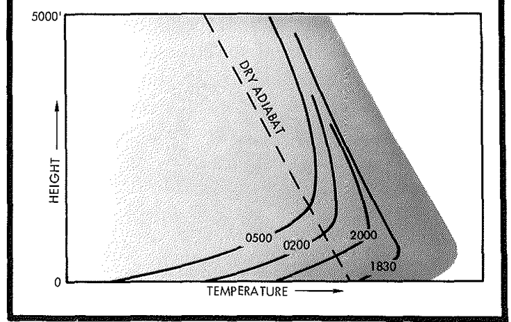
The ground cools rapidly after sundown and a shallow surface inversion is formed (1830). This inversion deepens from the surface upward during the night, reaching its maximum depth just before sunrise (0500).
