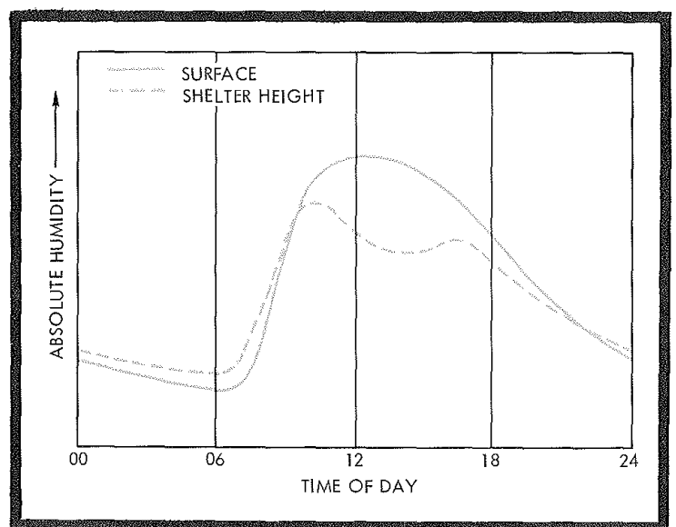
Schematic representation of surface absolute humidity compared to that at shelter height. Air near the surface is likely to contain less moisture than air at shelter height during the night, and more moisture during the day.
