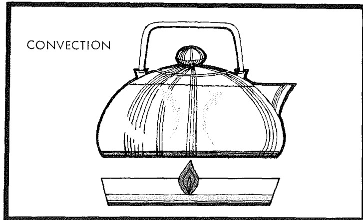
Heating a kettle of water sets up convection currents which transfer heat throughout the water.
