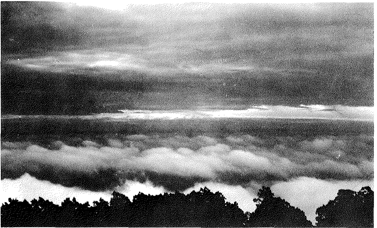
Nimbostratus is a gray or dark massive cloud layer diffused by more-or-less continuous rain or snow which usually reaches the ground. It is thick enough to blot out the sun. Lower ragged clouds often appear beneath the nimbostratus layer.
