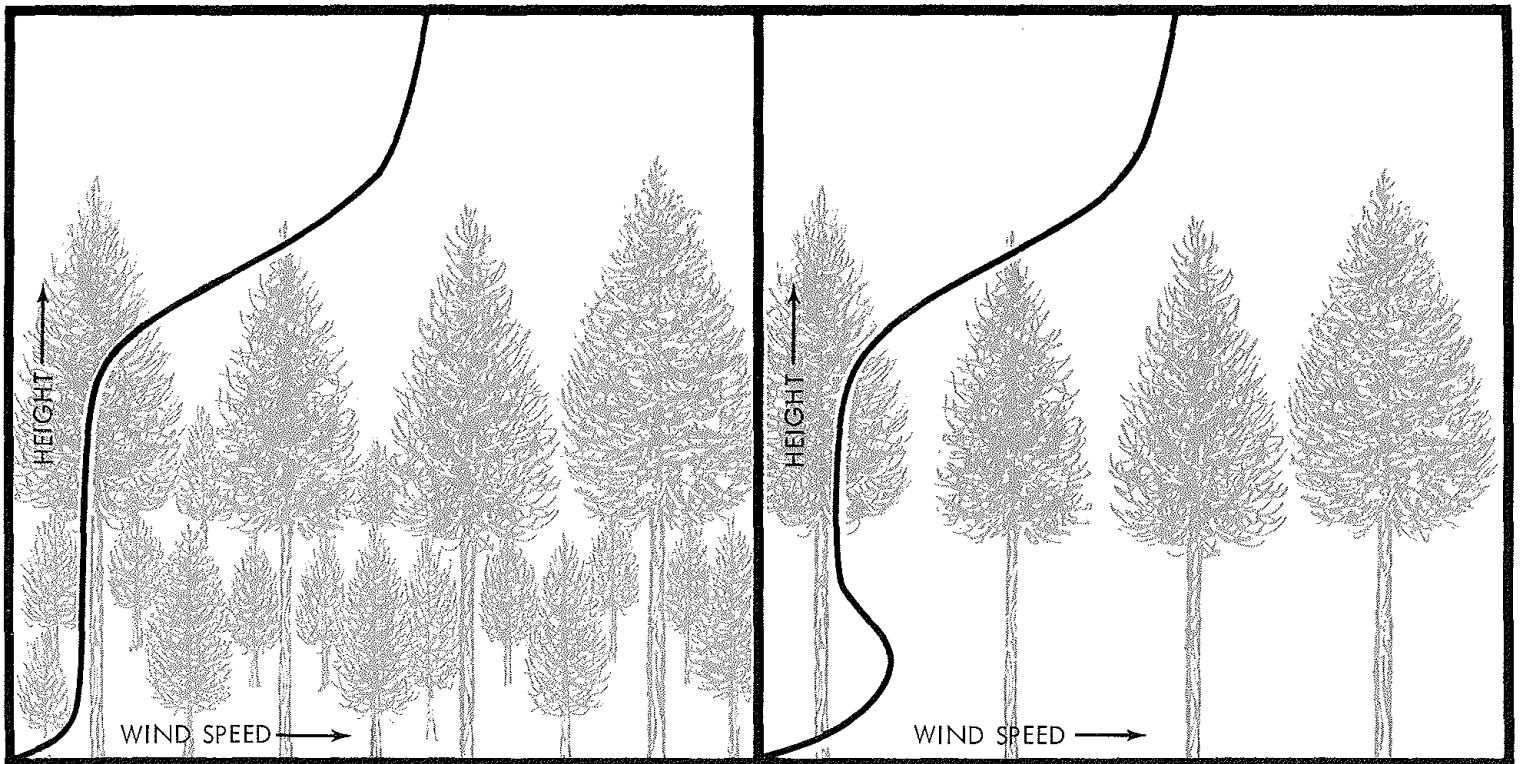
Vertical wind profiles in forest stands show that the crown canopy is very effective in slowing down wind movement. In stands with an understory, the wind speed is nearly constant from just above the surface to near the tops of the crowns. Above the crowns, wind speed increases much like above level ground. In stands with an open trunk space, a maximum in wind speed is likely in the trunk space and a minimum in the crown area.
