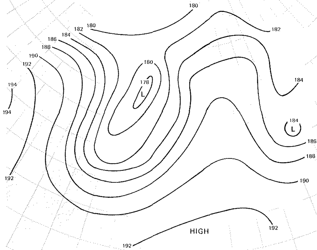
500 MB CHART
