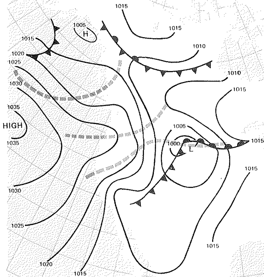
SEA-LEVEL CHART
