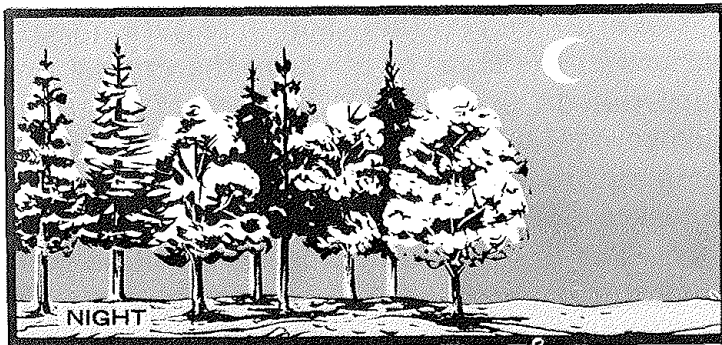
Relative humidity is normally higher under a closed canopy than in the open during the day, and lower at night.
