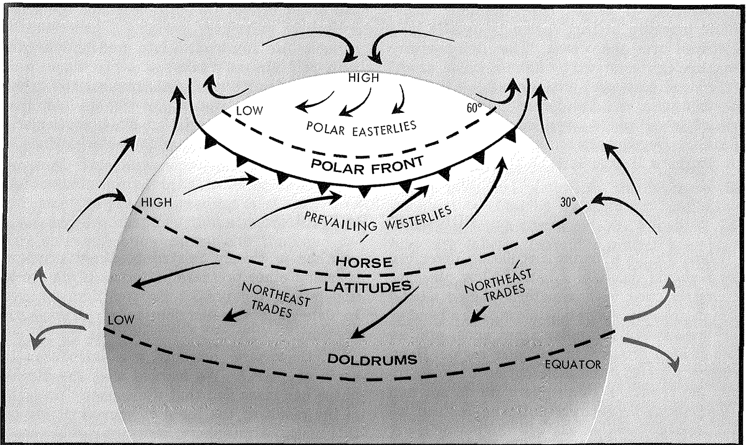
On a rotating earth with a uniform surface, the general circulation of the Northern Hemisphere would be composed of the northeast trade winds, prevailing westerlies, and polar easterlies.
