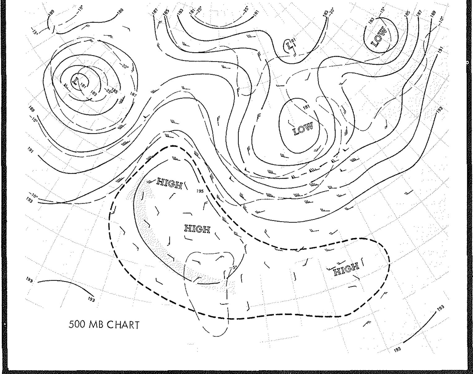
Moisture from the Gulf of Mexico is transported to the Southwest and the Western States at mid-tropospheric levels when a close High aloft moves into the position shown on this 500-mb. chart. Daytime heating and orographic lifting of the moist air combine to produce many high-level thunderstorms.
