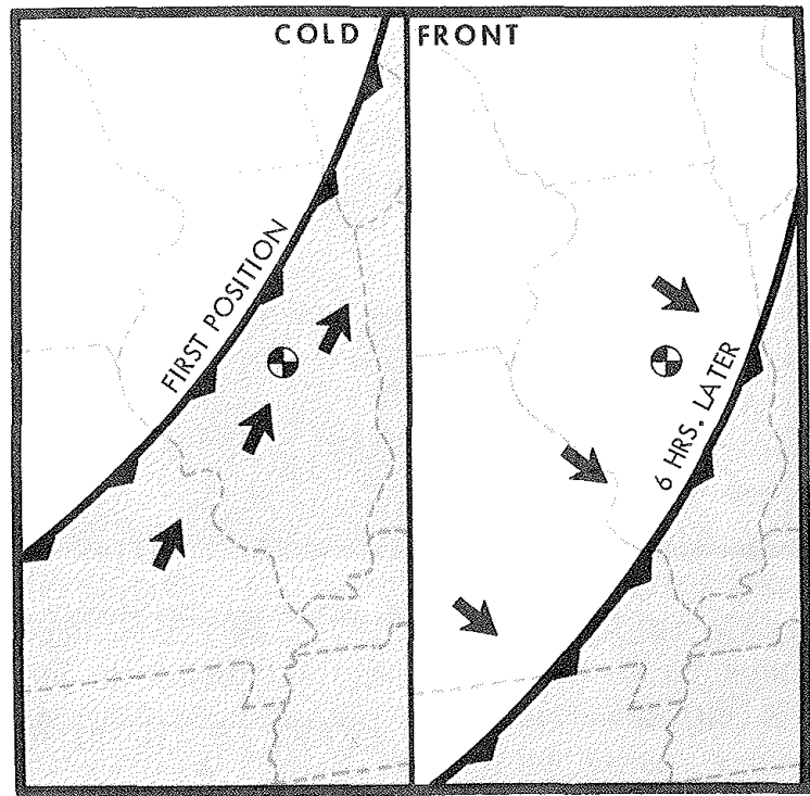
Winds increase ahead of a cold front, become gusty and shift abruptly, usually from a southwesterly to a northwesterly direction, as the front passes.
