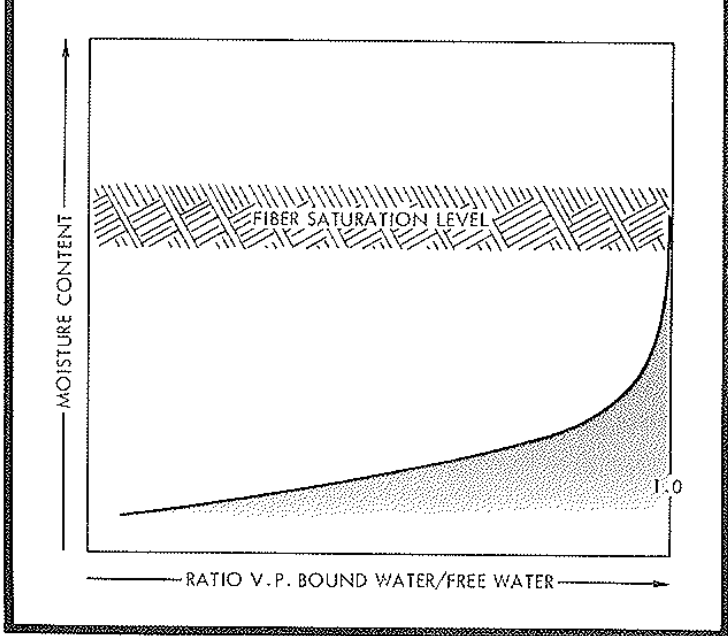
At moisture contents below the fiber-saturation level, the vapor pressure of bound water is less than that of free water. The ratio of these vapor pressures is unity at that level and decreases as moisture content decreases.
