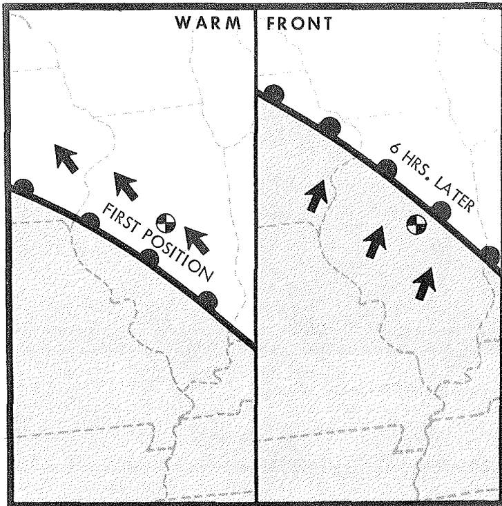
As a warm front passes, wind is steady and shifts gradually, usually from a southeasterly to a southwesterly direction.
