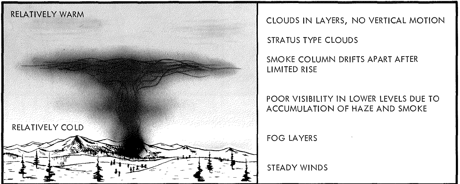
Visible indicators of a stable atmosphere.
