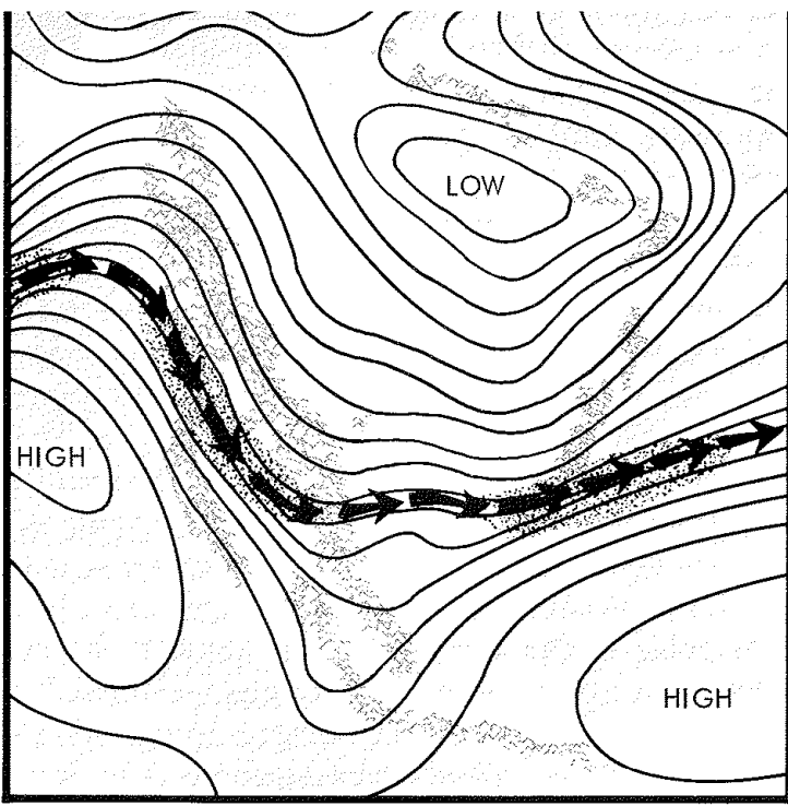
The jet stream, as shown on a constant-pressure chart in the upper troposphere, is a meandering, fast-flowing river of air embedded in the belt of westerlies. The stippling shows the regions of strongest winds that move along the jet stream.
