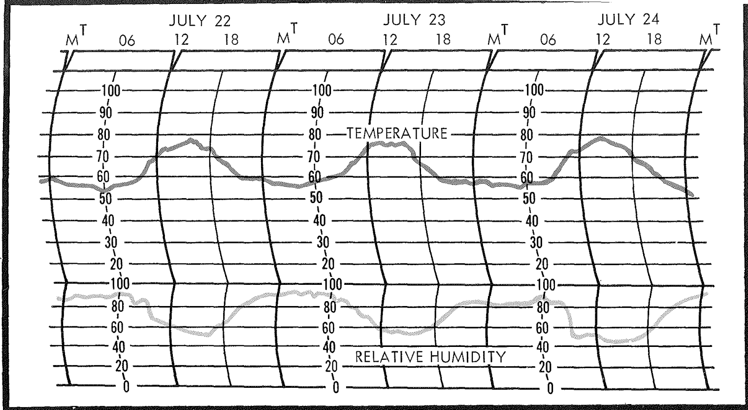
Typical temperature and relative humidity traces for a low-level station are nearly mirror images of each other.
