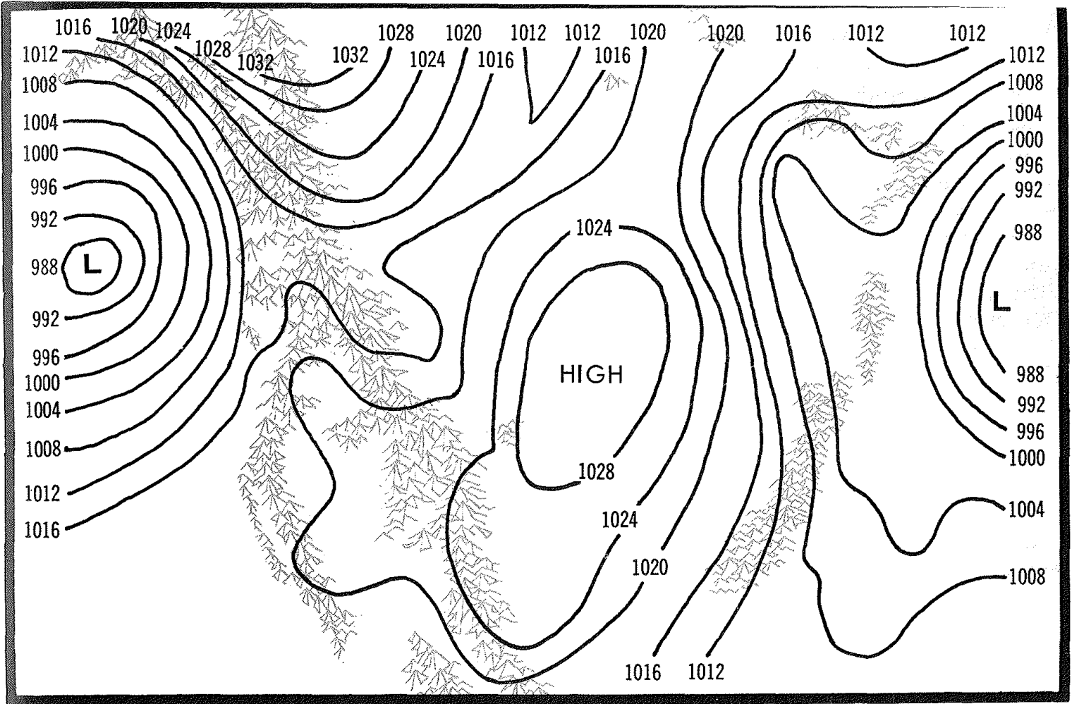
A surface weather map is a graphical picture of the pressure distribution obtained by drawing lines, called isobars, through points of equal sea-level pressure. Isobars outline areas of high and low pressure.
