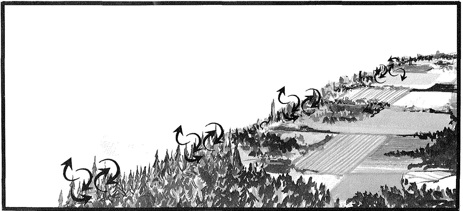
Squall lines produce violently turbulent winds, usually for a few minutes.
