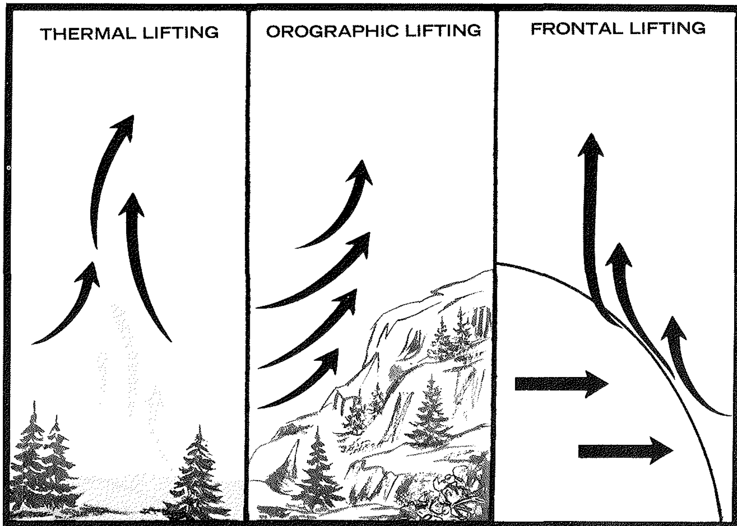
The most important method of cooling air to saturation is adiabatic cooling because of lifting. Lifting may be thermal, orographic, or frontal.
