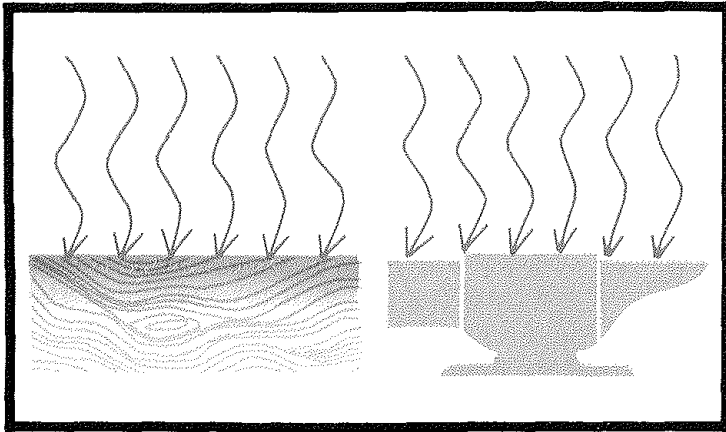
Top.—Surface materials differ in their absorptive and reflective properties. Dark pavements become quite hot in sunlight; dark soils become warmer than light soils. The temperature of tree crowns will rise also, but not as much. Center.—Heat absorbed by opaque substances, such as land, is concentrated in a shallow layer. Radiation penetrates deeply into water and warms a larger volume. Bottom.—Radiant energy absorbed by a good conductor, such as metal, is rapidly transmitted through the material, while that absorbed by a poor conductor, such as wood, tends to concentrate near the surface, and the surface becomes quite hot.
