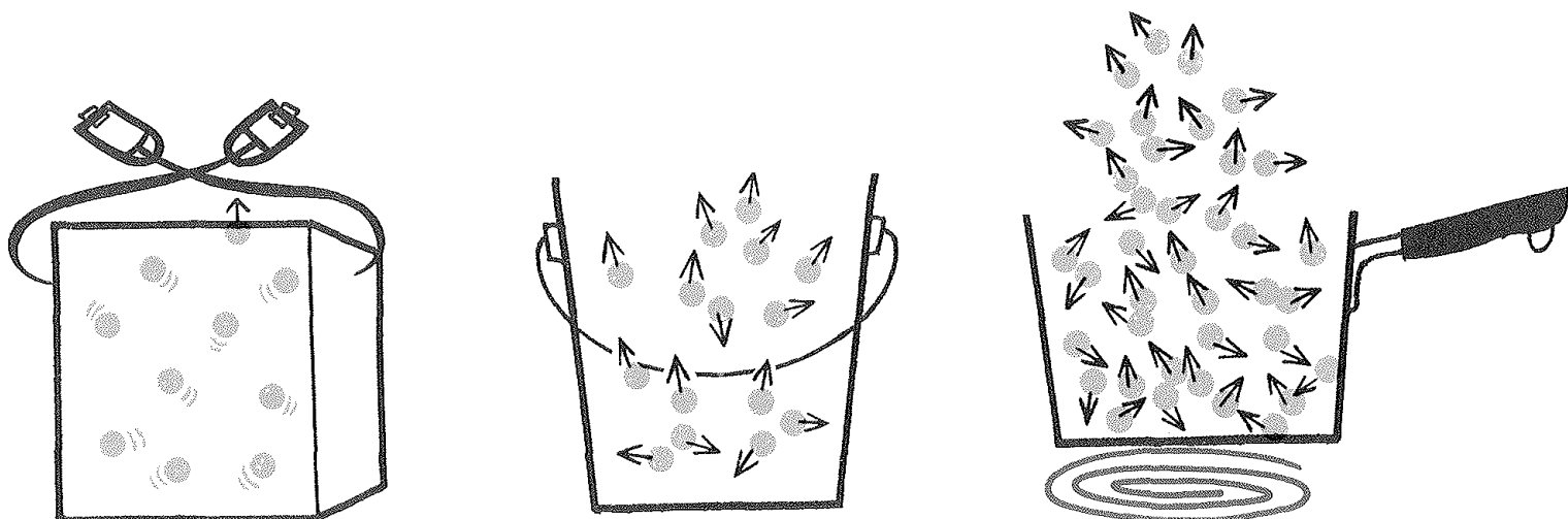
The internal pressure causing water vapor to escape from ice or liquid water varies greatly with the surface temperature; it is very small at cold temperatures and increases rapidly in liquid water through the boiling stage.
