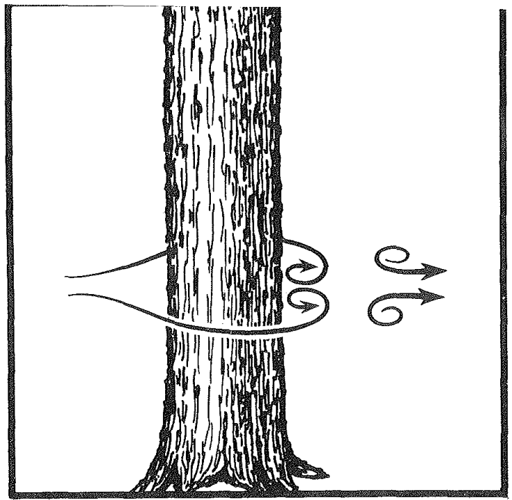
Local eddies form in the lee of each tree stem and affect the behavior of surface fires.
