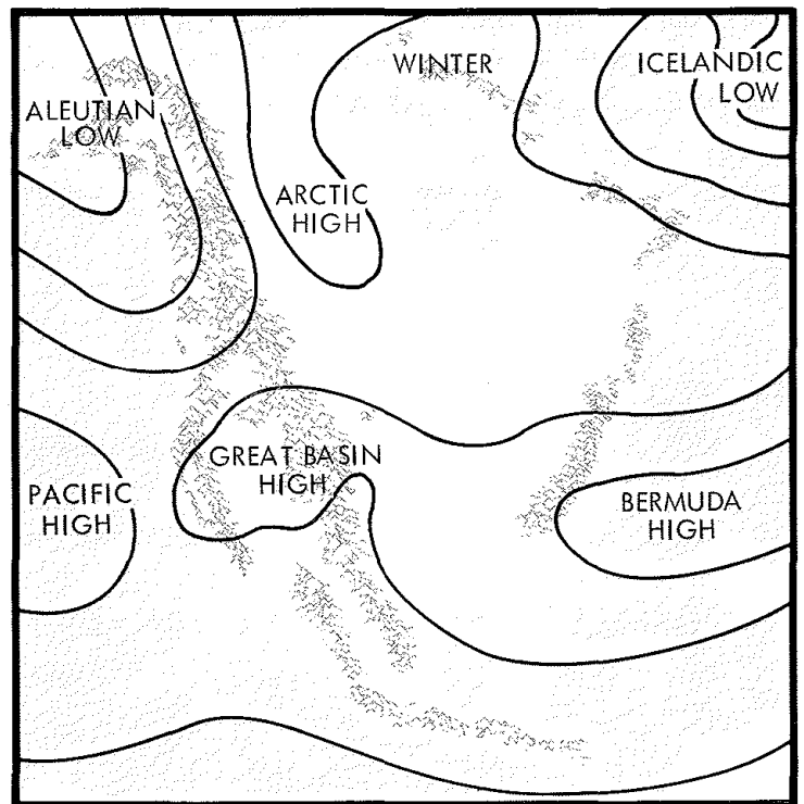
The average January sea-level pressure pattern, representing the winter pattern, shows that the Aleutian and Icelandic Lows are well developed. The Pacific and Bermuda Highs are weaker and farther south than in summer. Pressure is generally high over the cold continent, causing seasonal Highs such as the Great Basin High and the Arctic High to form.
