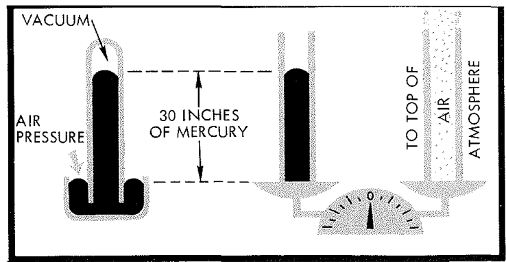
A column of air from sea level to the top of the atmosphere weighs about the same as a 30-inch column of mercury of the same diameter.
