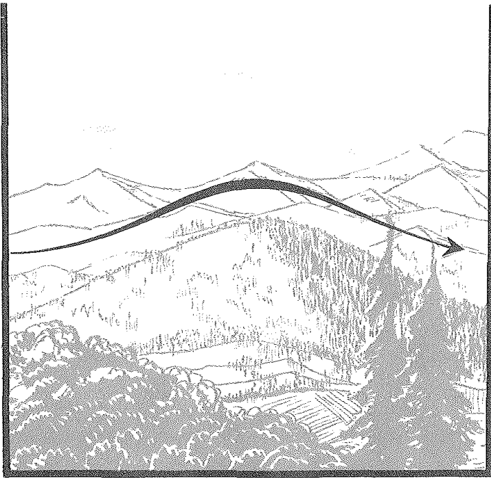
Airflow crossing a ridge is influenced by the ridge shape and by the wind speed and direction. Rounded hills disturb wind flow the least. In light to moderate winds, there may be no marked turbulence.
