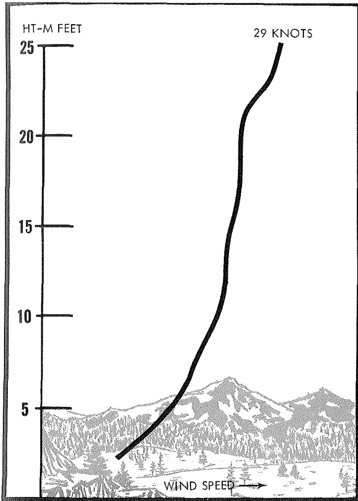
A wind profile without abrupt changes in wind speed or direction is characteristic of a well-mixed atmosphere.
