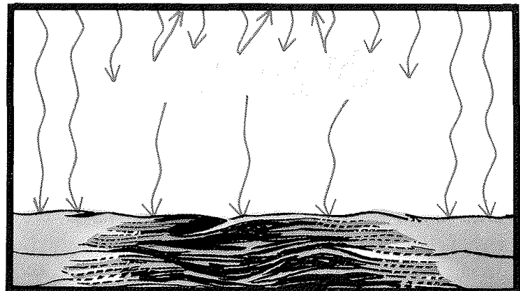
hours. South-facing slopes receive more nearly direct rays than do north-facing slopes. Upper right.—In open stands of timber, surface temperatures vary considerably from shaded to sunlit areas. Lower right.—Clouds both absorb and reflect incoming radiation and thereby reduce surface temperatures.
