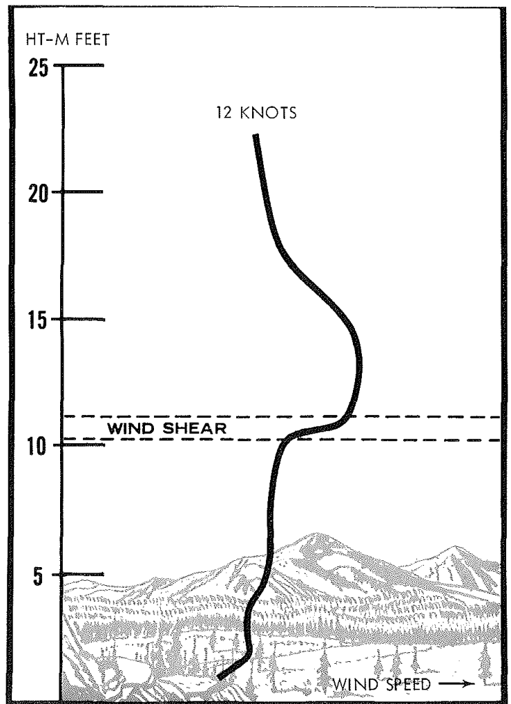
Wind shear occurs where wind speeds change abruptly.
