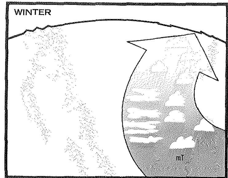
Maritime tropical air in winter produces nighttime cloudiness and fog in the Mississippi Valley and Great Plains and showers or snow over the Appalachians and in areas where it overruns a cooler air mass.
