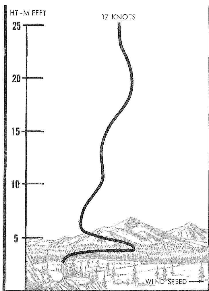
Low-level jets occur predominately in night wind profiles in the Plains, but they may also occur elsewhere. The jet is found most frequently just above the night inversion.
