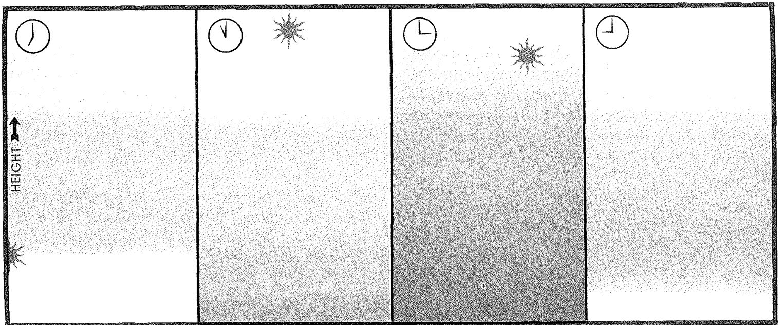
On a typical fair-weather summer day, stability in the lower atmosphere goes through a regular cycle. Cooling at night near the surface stabilizes the layer of air next to the ground. Warming during the daytime makes it unstable.
