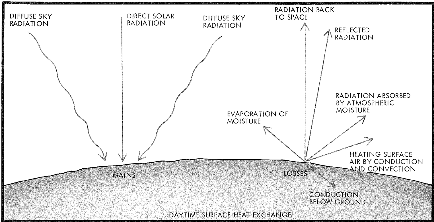
Solar radiation that reaches the earth's surface during the daytime is dissipated in several ways.
