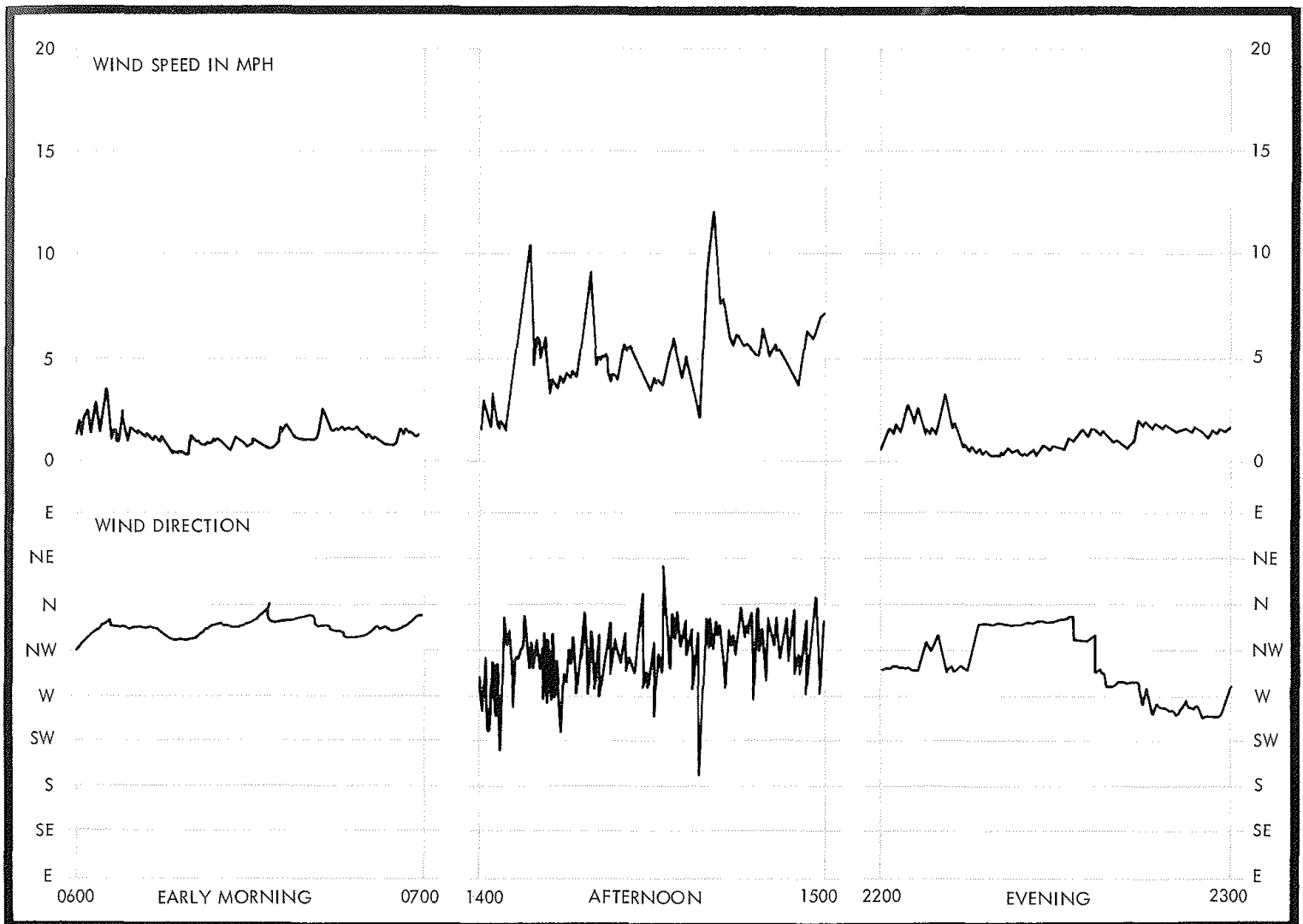
On clear days over flat terrain, thermal turbulence, as indicated by the fluctuations in wind speed and direction, shows diurnal changes because of day heating and night cooling. Turbulence is most pronounced in early afternoon when surface heating is maximum and the lower layers of air are unstable, and least pronounced during the night and early morning when the air is stable.
