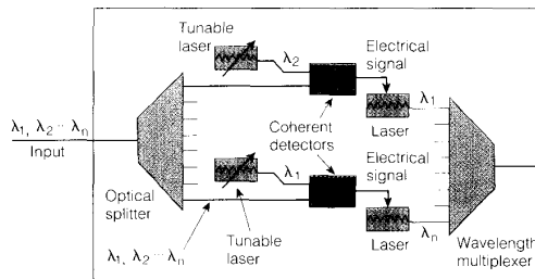
[2] In wavelength interchanger, a multiwavelength input is divided among many coherent detectors. Heterodyned by a tunable laser, each coherent detector extracts an electrical modulation signal representing a discrete input wavelength and uses it to modulate a laser operating at a different wavelength. Any input wavelength can be switched to any output wavelength.
