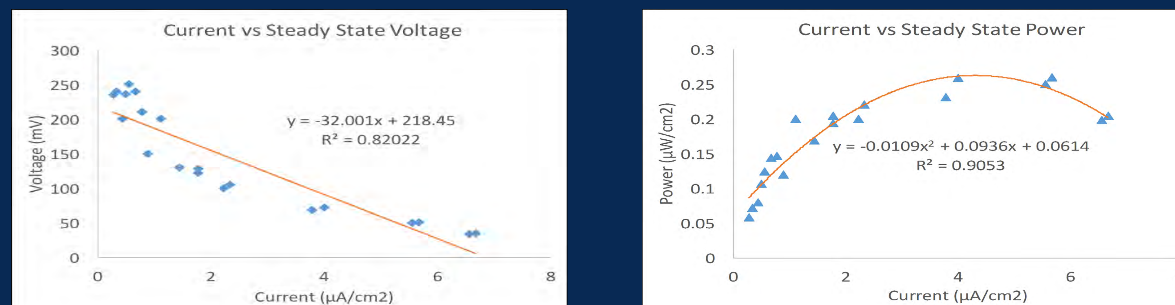
Figure 3: Voltage and power generation from simple design
