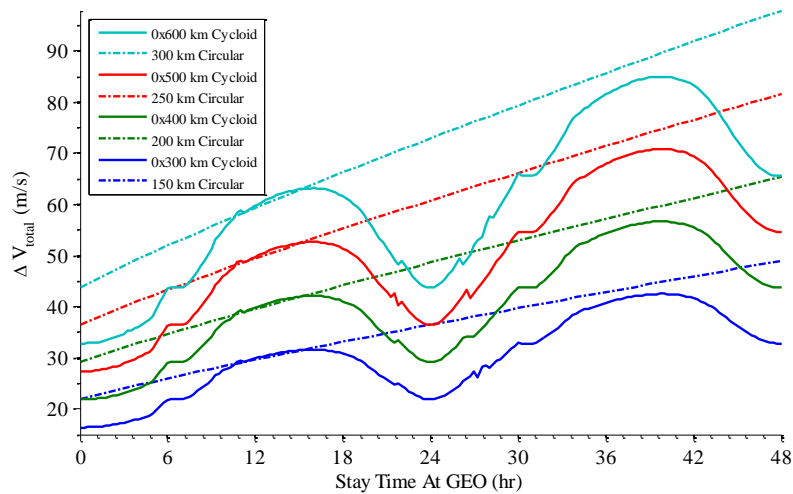
Figure 3 – Optimal roundtrip in-plane delta-v requirements for a Carrier SmallSat inspection sortie as a function of GEO stay-time/inspection-time. The dash-dot curves show delta-v requirements for different circular Carrier orbits with synodic periods ranging from 3 months to 6 months. The solid curves show delta-v requirements for different cycloid orbits with the same range of synodic periods.
