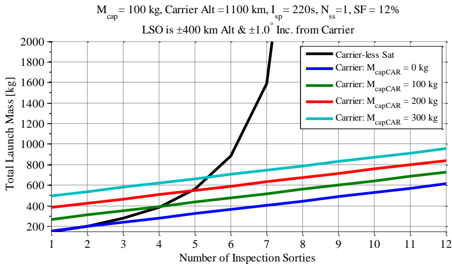
Figure 10 – Launch mass as a function of the number of LEO inspection sorties for a SmallSat Carrier concept and a carrier-less SmallSat concept.
