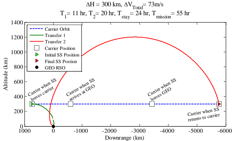
Figure 2 – Example Carrier SmallSat (SS) rendezvous trajectory for a short 55 hour sortie. The dashed blue line is the position of the Carrier relative to the GSO (black dot) at the origin. The white squares are the position of the carrier at different times in the mission. The green curve is the transfer from the carrier to the GSO. The red curve is the transfer of the SS from the GSO to the Carrier.
