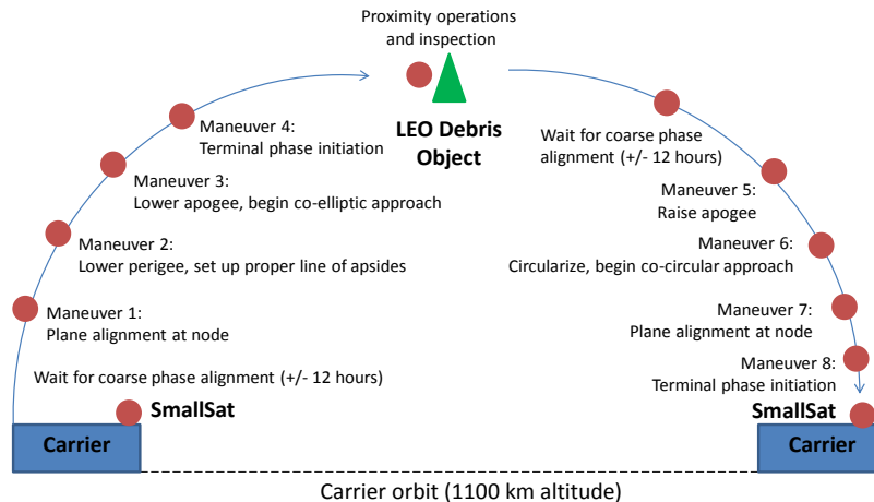
Figure 7 – Example of Carrier SmallSat rendezvous maneuver sequence for a LEO inspection sortie
