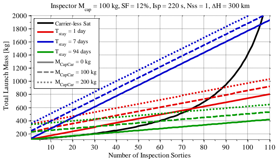
Figure 5 – Launch mass as a function of the number of GEO inspection missions for both a Carrier concept and carrier-less concept
