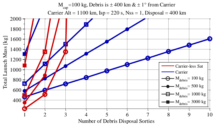
Figure 11– Launch mass as a function of the number of LEO debris sorties for a SmallSat Carrier concept and a carrier-less SmallSat concept.
