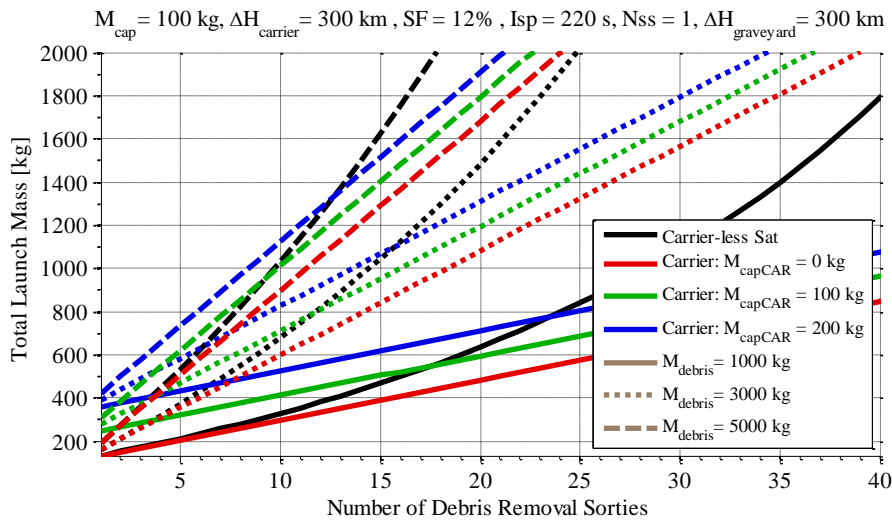
Figure 6 – Launch mass as a function of the number of GEO debris disposal sorties for both a SmallSat Carrier concept and a carrier-less SmallSat concept
