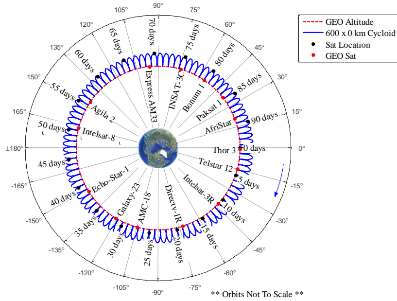
Figure 1 Carrier and GSO orbits in an Earth Centered Earth Fixed (ECEF) reference frame. Top - Carrier orbit in a co-planar, co-circular orbit, 300 km above GEO. Bottom - Carrier in a cycloid orbit with apogee 600 km above GEO and perigee at GEO altitude. The black dots represent the position of the carrier satellite as a function of time. The red dots are fixed GSO locations. The red dotted line is the geostationary orbit. The blue line is the orbit of the Carrier in an Earth Centered Earth Fixed (non-inertial) reference frame. The figure shows that it takes about 94 days for the carrier to return to the same GEO longitude.
