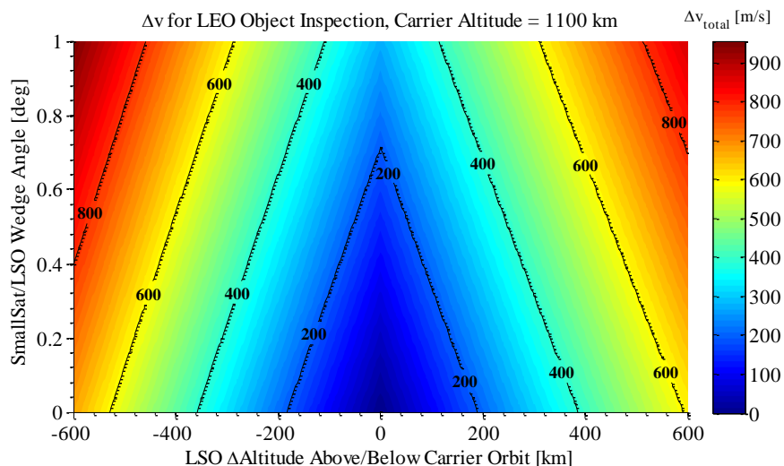
Figure 8 – Required Carrier SmallSat delta-v for a roundtrip inspection sortie as a function of key LEO space object orbital parameters (wedge angle and altitude). Results will be similar for a carrier-less SmallSat.
