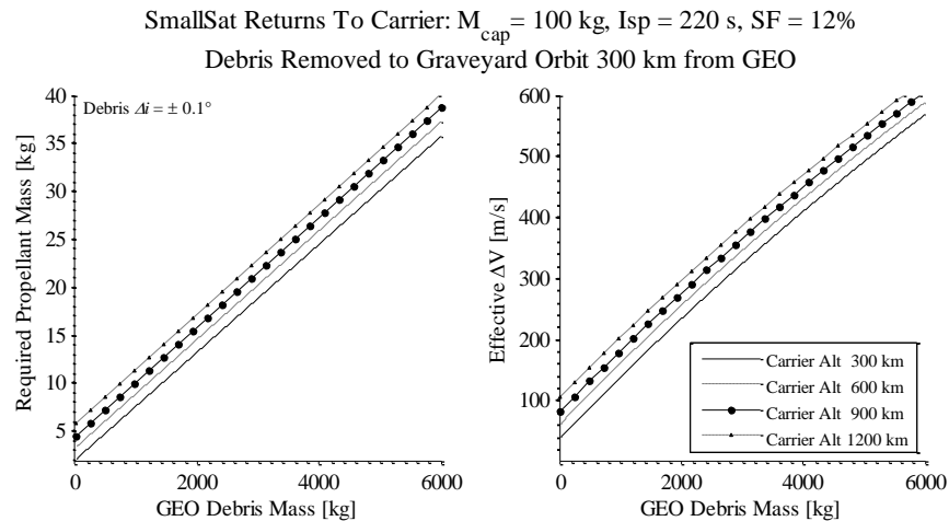
Figure 4 – Required SmallSat propellant mass (left) and effective delta-v (right) as a function of GEO debris object mass and Carrier altitudes ranging from 300 km to 1200 km (and synodic periods ranging from 1 week to 3 months)
