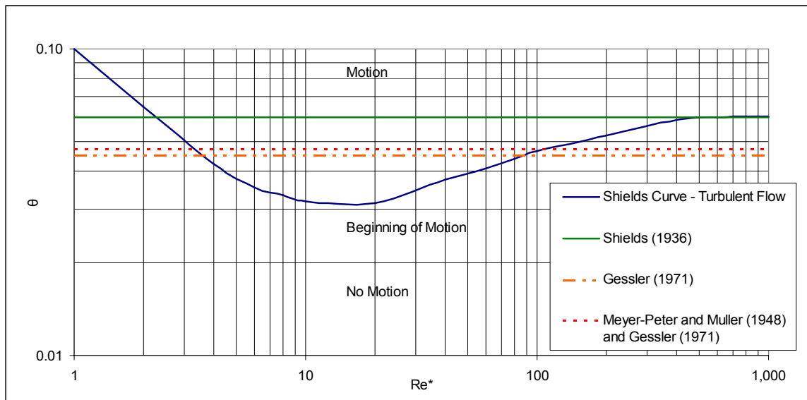
Figure 2. Shields relation for beginning of motion.
