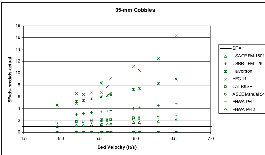
Figure 66. Comparison of riprap safety factors for 2-inch cobbles in a rectangular flume.
