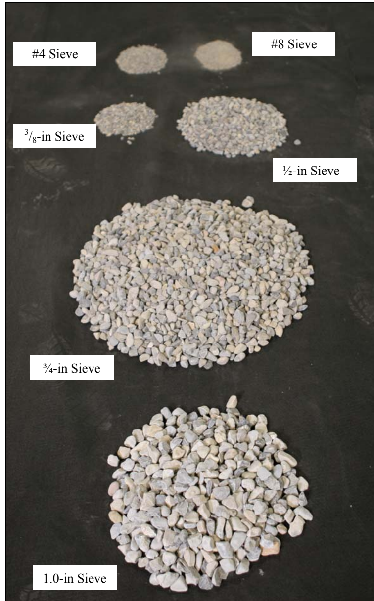
Figure G2. Sieve distribution of 0.75-inch angular gravel substrate
