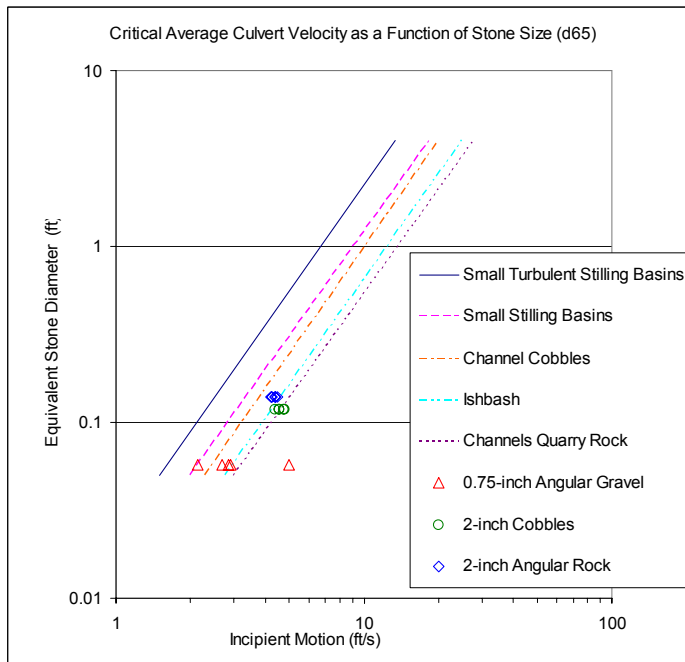
Figure 25. Critical average culvert velocity as a function of stone size ‡ .
