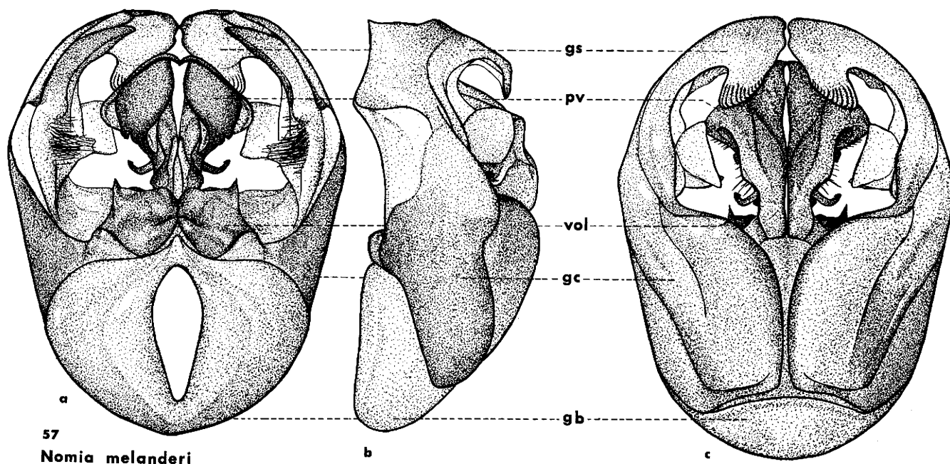
FIGURE 57. Genital capsule of Nomia melanderi male: (a) ventral view, (b) lateral view, and (c) dorsal view (gb = gonobase; gc = gonocoxite; gs = gonostylus; pv = penis valve; and vol = volsella).
