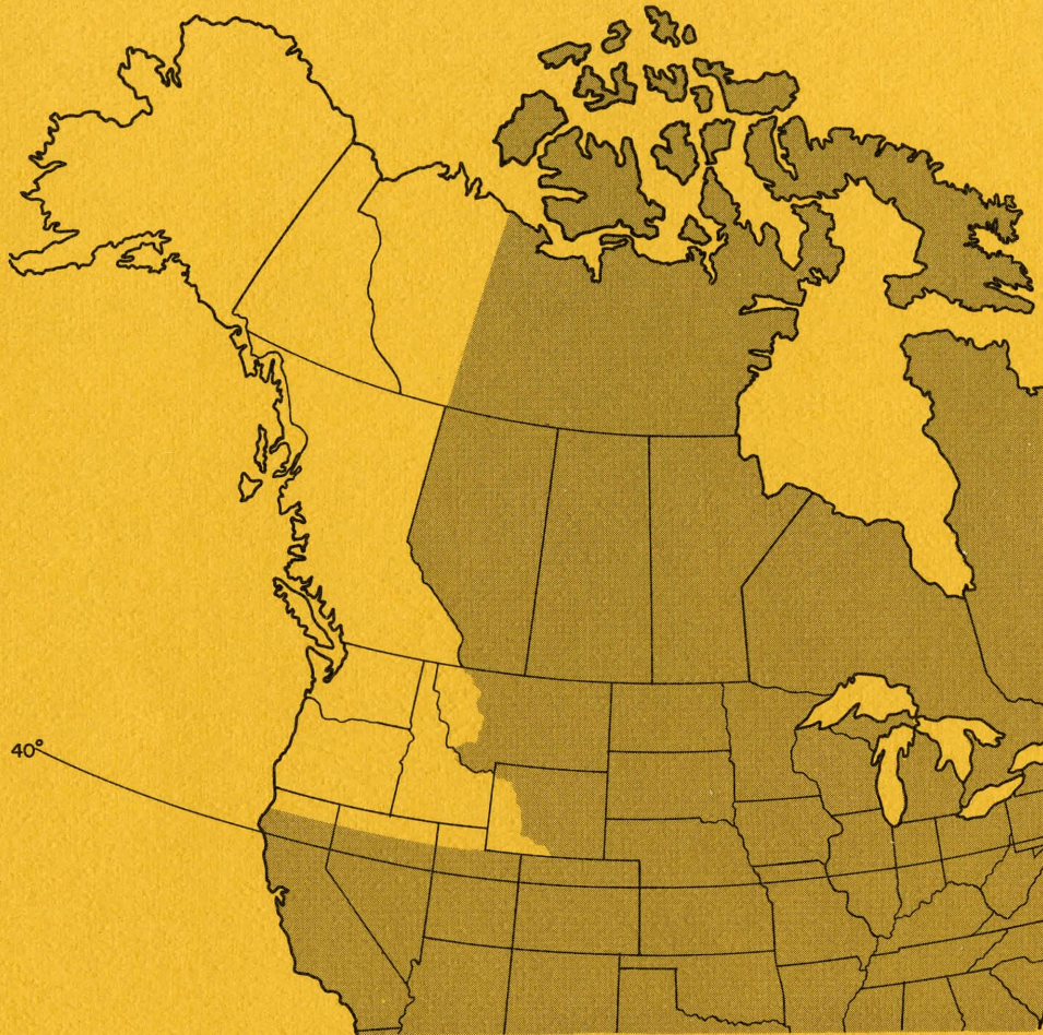
Northwestern America as interpreted for taxonomic synopses.
