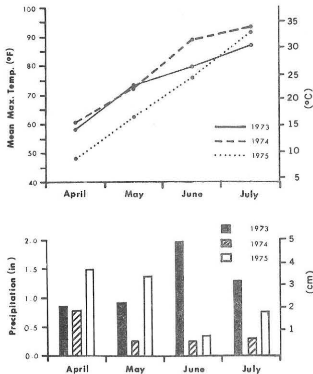
Figure 2. Mean monthly maximum temperature and precipitation recorded at Snowville station for 1973, 1974 and 1975.
