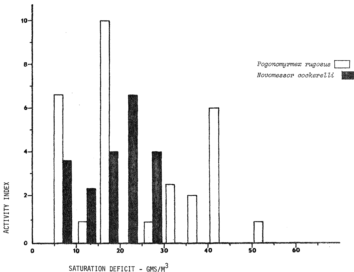
Figure 3. The influence of saturation deficit on foraging activity of two species of harvester ants. Activity index equals the number of foragers returning to the nest in four minutes.
