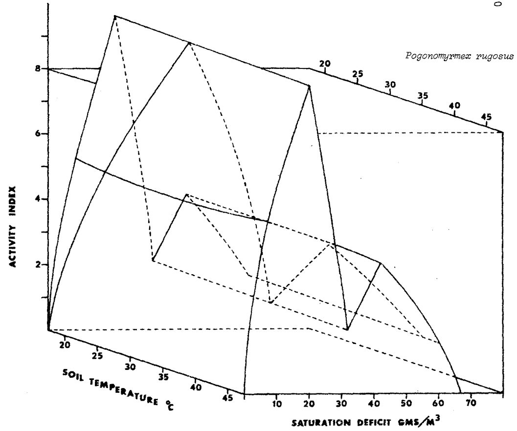
Figure 5. Soil temperature-saturation deficit levels at which Pogonomyrma rugosus forage.
