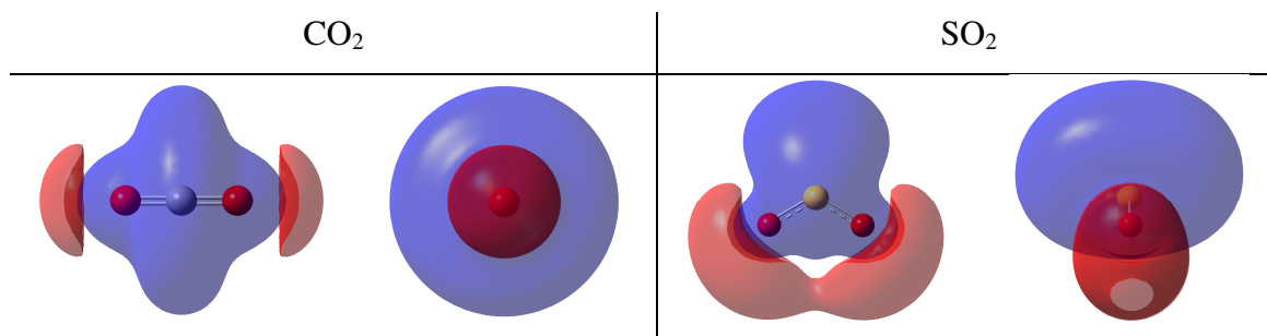
Figure 1. Molecular Electrostatic Potential (MEP) for the monomers \text{CO}_2 and \text{SO}_2 at the \pm 0.020 au contour at the MP2/aug-cc-pVDZ computational level. Lefthand diagram represents molecular plane, and the normal plane is shown on the right. Red and blue regions indicate negative and positive regions, respectively.
