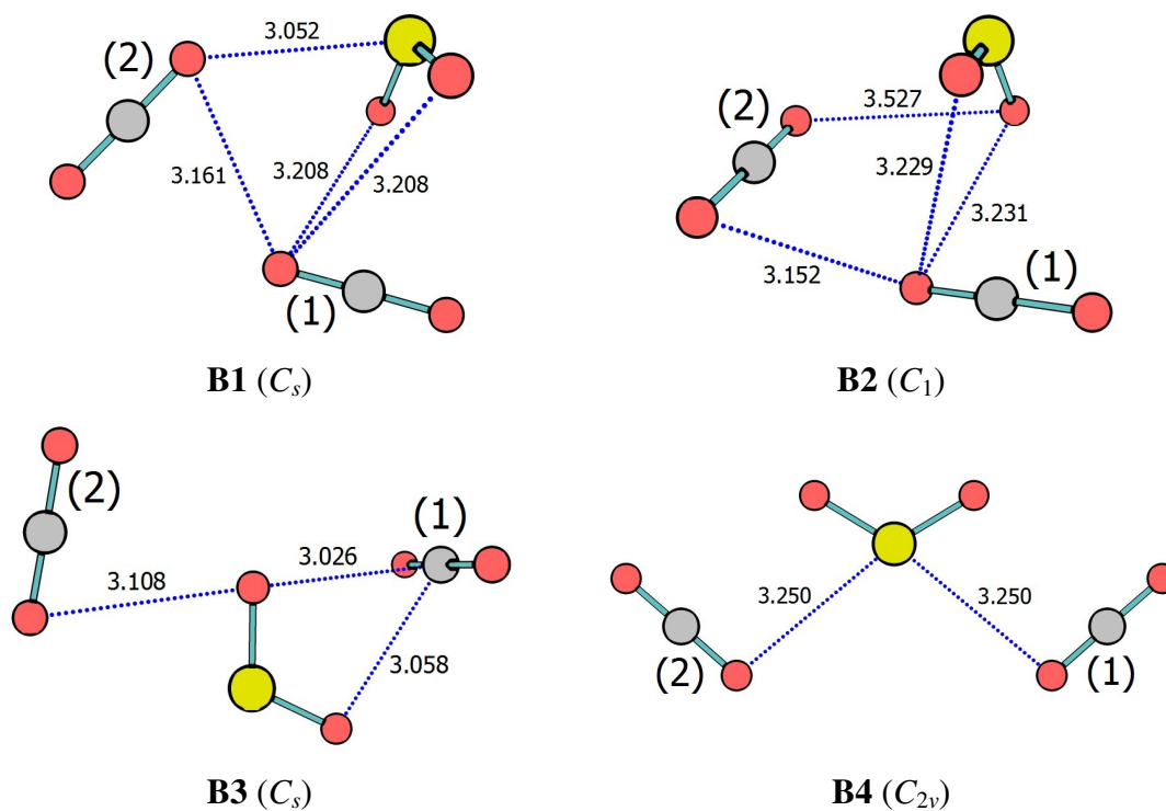
Figure 5. (CO 2 ) 2 :SO 2 heterotrimers optimized at MP2/aug-cc-pVDZ computational level. Broken blue lines link atoms which present interatomic AIM BCPs, with interatomic distances in Å. Complexes are arranged in ascending order of energy.
