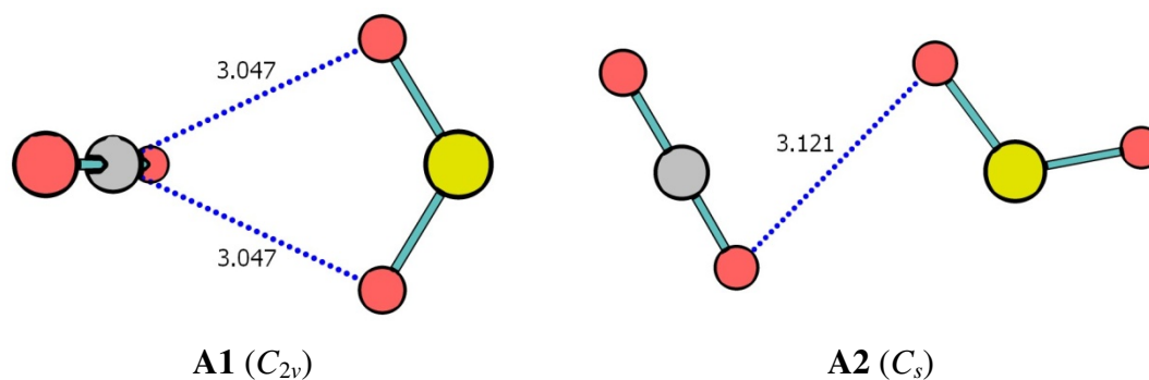
Figure 2. \text{CO}_2:\text{SO}_2 heterodimers optimized at the MP2/aug-cc-pVDZ computational level. Blue dotted lines link atoms which present interatomic AIM BCPs, with interatomic distances in Å. Complexes are arranged in ascending order of energy.
