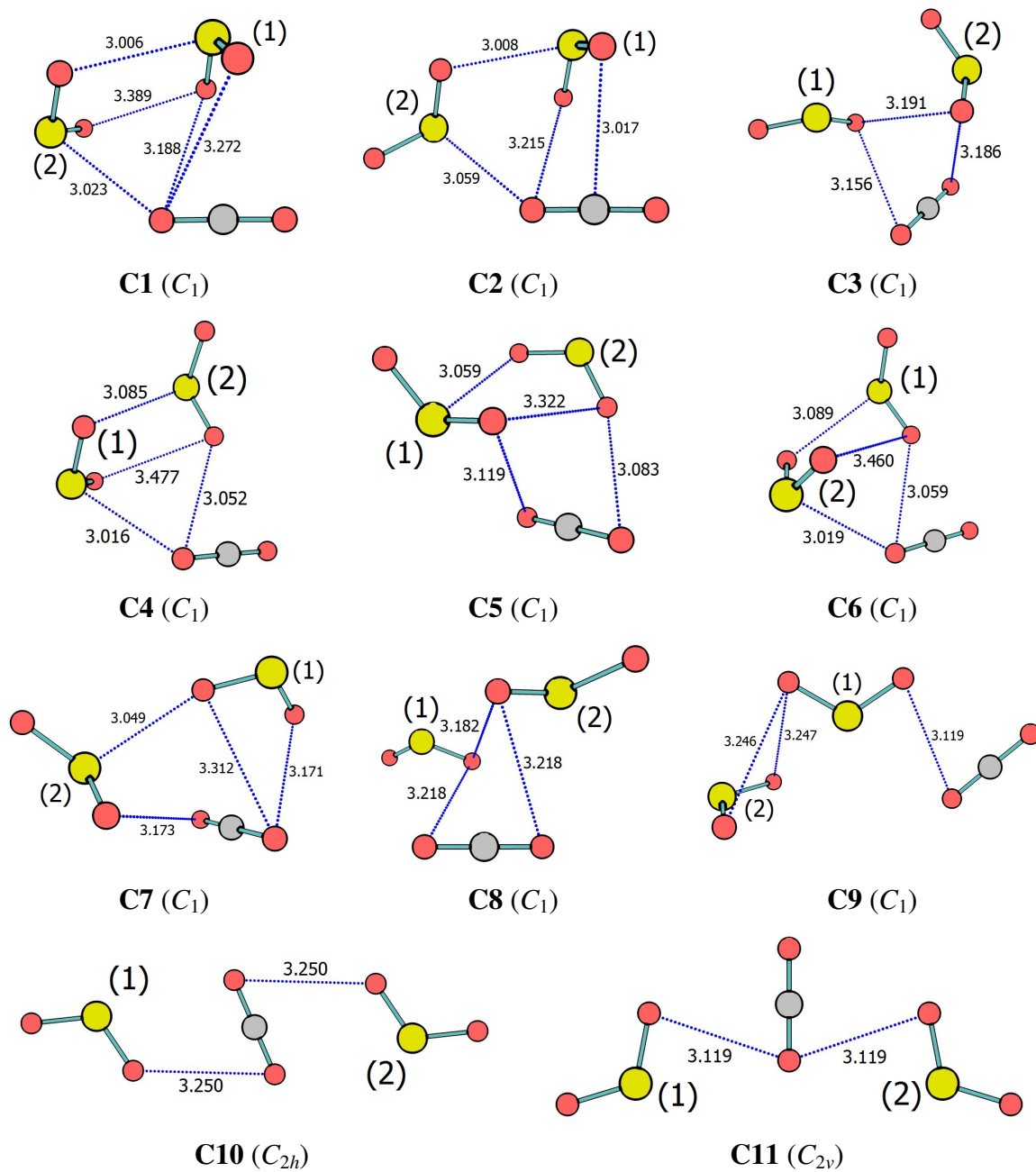
Figure 6. \text{CO}_2:(\text{SO}_2)_2 heterotrimers optimized at the MP2/aug-cc-pVDZ level. Blue broken lines link atoms which present interatomic AIM BCPs, with interatomic distances in Å. Complexes are arranged in ascending order of energy.
