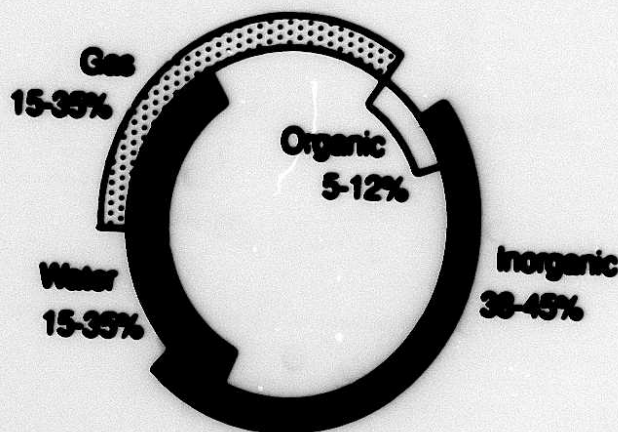
Figure 1. Typical Volumetric Composition of Soil.
