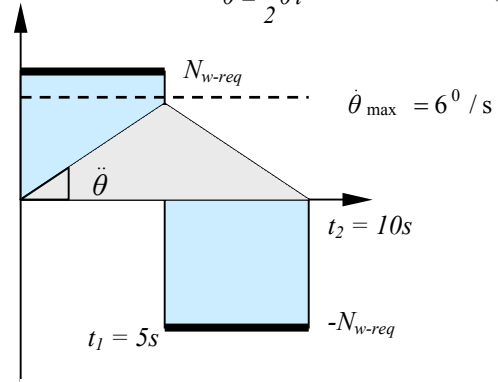
Figure 5: Torque and acceleration diagram for an SSTL microsattellite executing a 30^0 manoeuvre in 10 seconds
