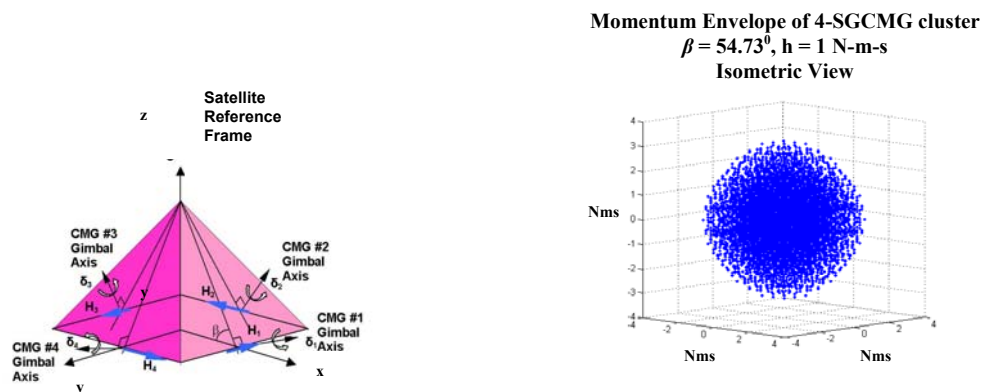
Figure 4: 4-SGCMG cluster in pyramid arrangement and momentum envelope
