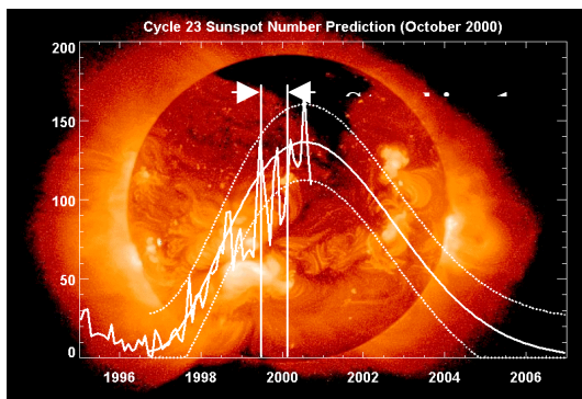
Figure 2 Sunspot Number Plot for 1 st Half Solar Cycle 23
