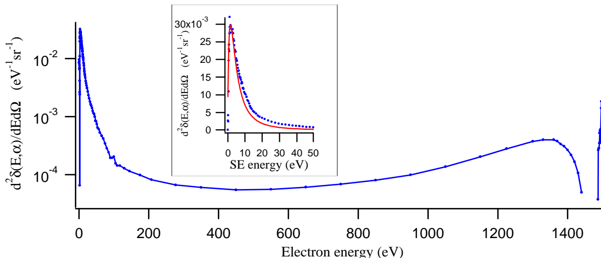
Figure 2. Energy-distribution of secondary and backscattered electrons at an emission angle of 17° measured for polycrystalline gold with 1500 eV primary electron beam energy [Davies, 1999a]. Note the logarithmic axis for the number of electrons. Inset shows a comparison of the low energy secondary electron energy-distribution (circles) fit with the theoretical model of Eq. 1 (solid line) [Chung and Everhart, 1974].
