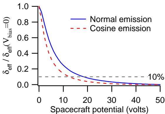
Figure 4. Effective SE yield (as a percentage of the unbiased SE yield) as a function of positive spacecraft potential for fully normal (solid line) and cosine (dashed line) SE angular-distributions. Sample is polycrystalline gold.
