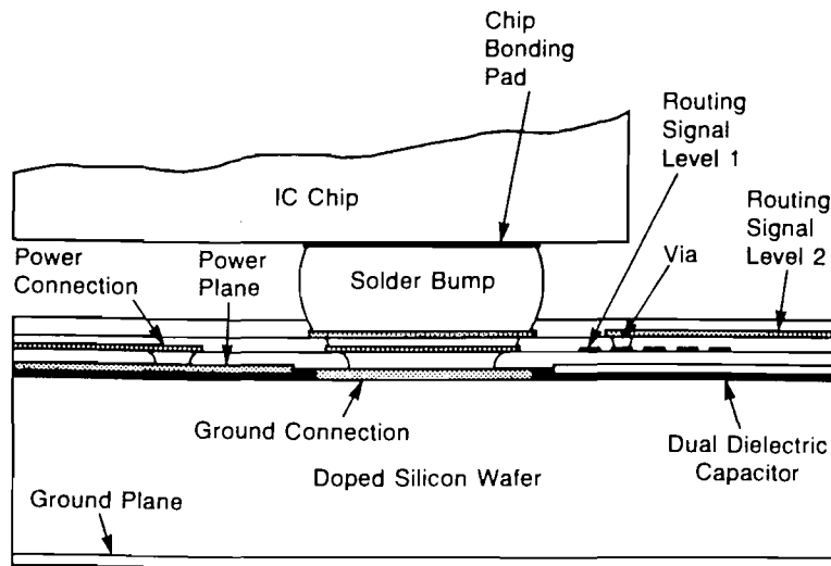
Figure 3. Cross-section of HWSI Substrate with Flip-Chip Bonded IC.
