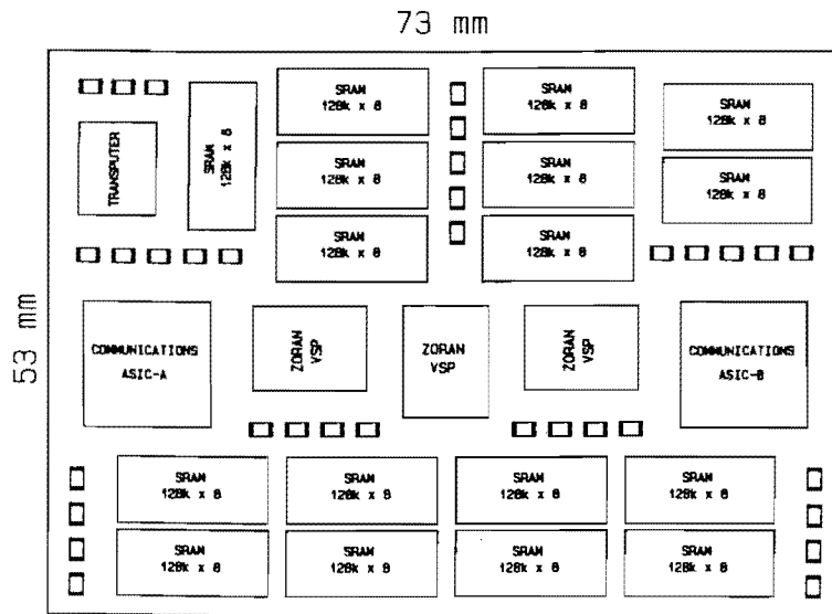
Figure 4. Component Placement on HWSI Substrate.
