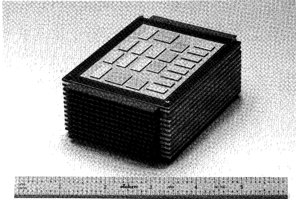
Figure 1. Full Scale Model of Miniaturized Space Processor with Cover Removed. (Throughput = 1.2 GFLOPS)
