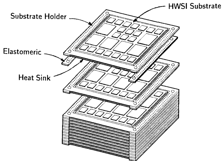
Figure 5. 3-D Stack Technology.
