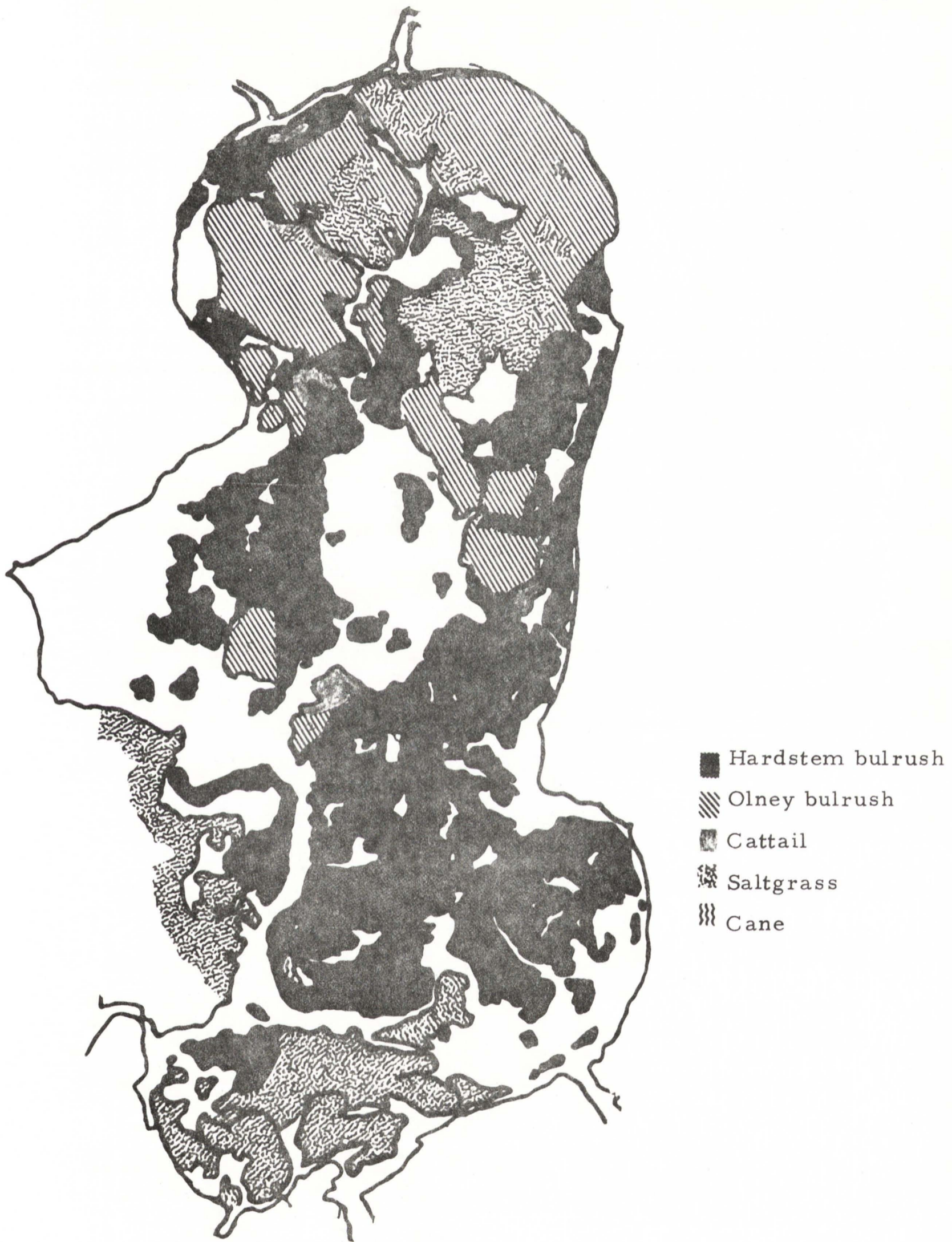
Figure 4. Knudson Marsh, Utah, 1975, showing cover types and open water.
