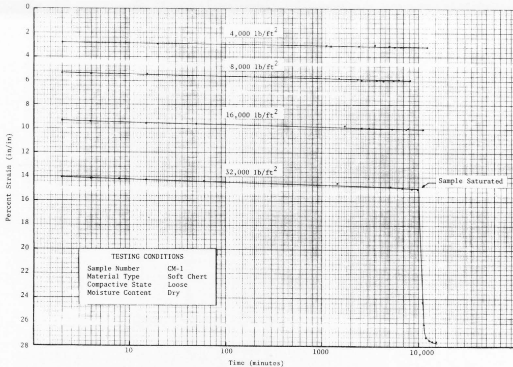
Figure III-24. Time versus compression characteristics of soft chert showing effect of saturation after reaching a stress level of 32,000 lb/ft 2 (1b/ft 2 = .0479 kPa).
