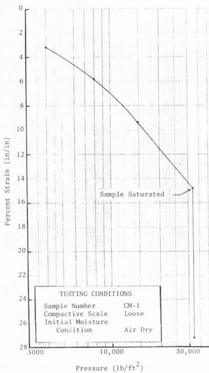
Figure III-25. Strain log pressure relationship for soft chert showing effects of saturation at a stress level of 32,000 lb/ft 2 (1 lb/ft 2 = .0479 kPa).
