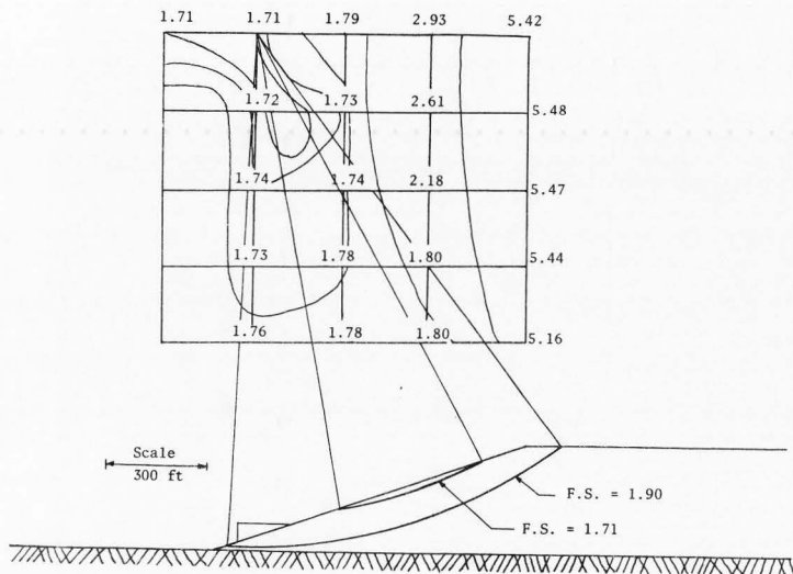
Figure IV-6. Contours of safety factors showing deep and shallow failures in waste shale embankments. (1 ft = 0.305 m)
