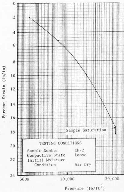
Figure III-32. Strain versus log pressure relationship for hard chert showing effect of saturation at a stress level of 32,000 \text{ lb/ft}^2 ( 1 \text{ lb/ft}^2 = .0479 \text{ kPa} ).
