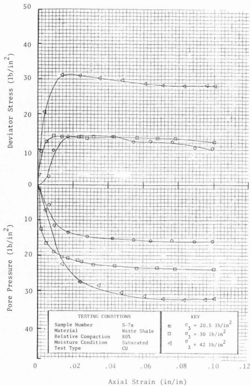
Figure III-59. Consolidated-undrained triaxial shear test stress-strain curves with pore pressure measurements ( 1 \text{ lb/in}^2 = 6.9 \text{ kPa} ).
