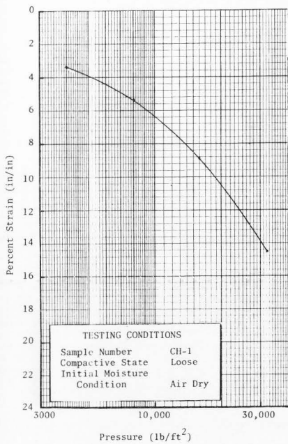
Figure III-31. Strain versus log pressure relationship for hard chert material subjected to cycles of wetting and drying ( 1 \text{ lb/ft}^2 = .0479 \text{ kPa} ).
