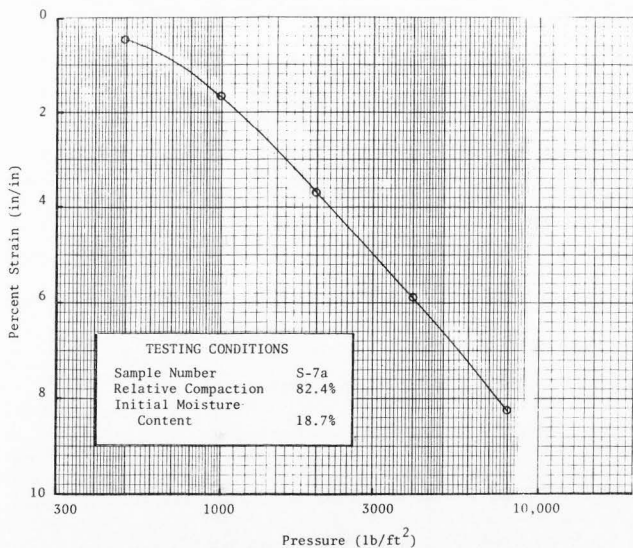
Figure III-40. Strain versus log pressure relationship for waste shale material compacted at 82.4% RC ( 1 \text{ lb/ft}^2 = .0479 \text{ kPa} ).
