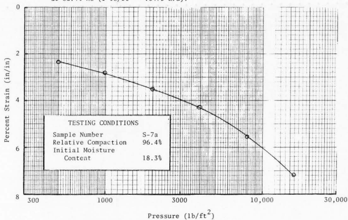
Figure III-41. Strain versus log pressure relationship for waste shale compacted at 96.4% RC ( 1 \text{ lb/ft}^2 = .0479 \text{ kPa} ).
