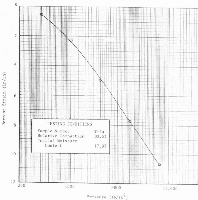
Figure III-59. Strain versus log pressure relationship for top soil material compacted at 83.6% RC (1 lb/ft 2 = .0479 kPa).
