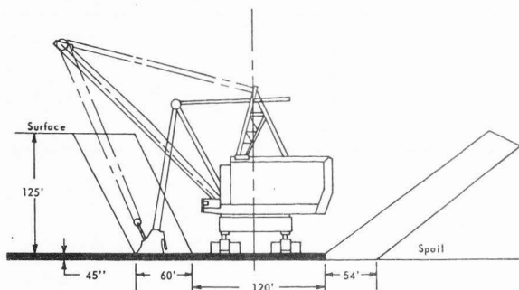
Section View
