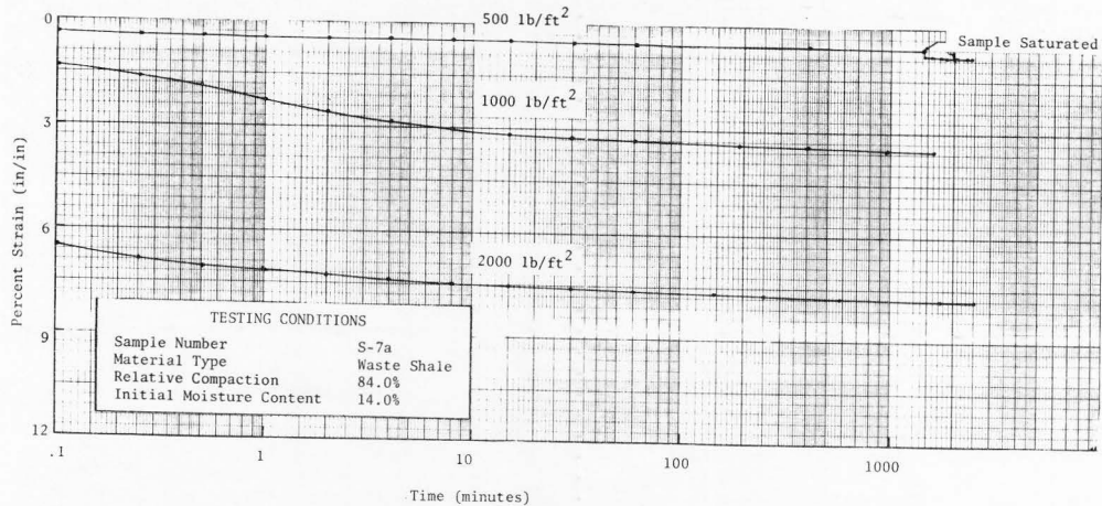
Figure A-8. Time-compression characteristics of waste shale material showing effect of saturation at a stress level of 500 lb/ft 2 (1 lb/ft 2 = .0479 kPa).
