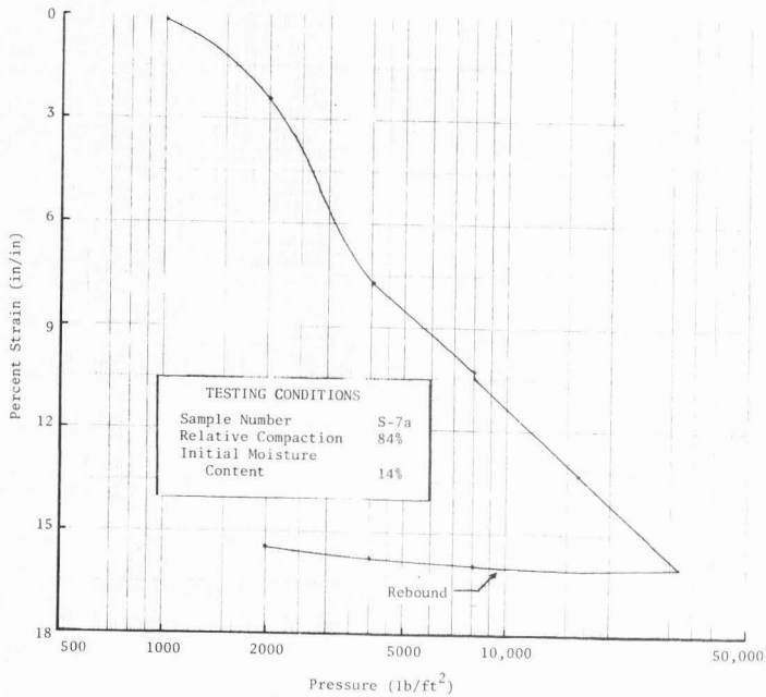
Figure III-37. Strain versus log pressure relationship for waste shale material showing effect of increasing the moisture content at low pressures ( 1 \text{ lb/ft}^2 = .0479 \text{ kPa} ).
