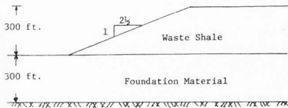
Figure IV-2. Cross-section of example problem illustrating the effect of weak foundation soils (1 ft = 0.305 m).
