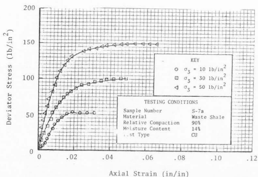
Figure III-54. Consolidated-undrained triaxial shear test stress-strain curves for partially saturated samples ( 1 \text{ lb/in}^2 = 6.9 \text{ kPa} ).
