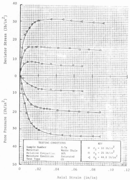
Figure III-62. Consolidated-undrained triaxial shear test stress-strain curves with pore pressure measurements (1 lb/in 2 = 6.9 kPa).
