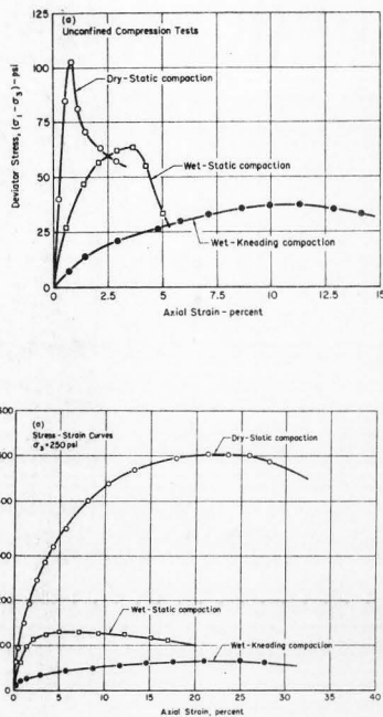
Figure II-3. Unconfined compressive strength and unconsolidated undrained strength characteristics of Higgins Clay (after Lee and Haley, 1968).
