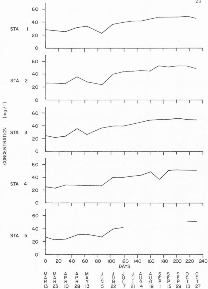
FIGURE 6 Variations in Total Carbon Concentrations with time in Summit Creek
