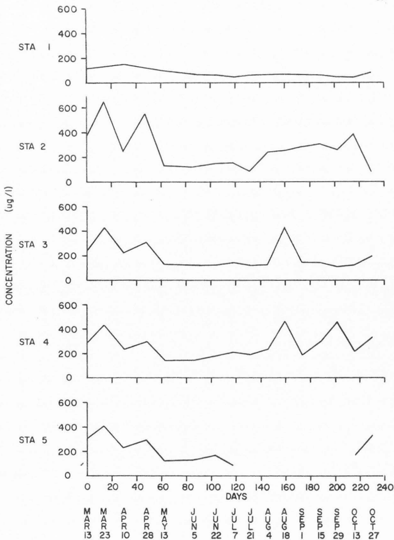
FIGURE 13 Variations in Nitrate Nitrogen Concentration with time in Summit Creek
