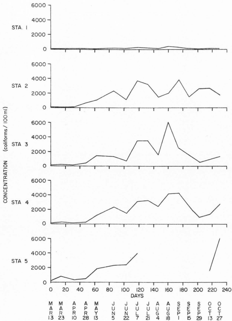
FIGURE 2 Variations in Concentration of Total Coliforms with time in Summit Creek
