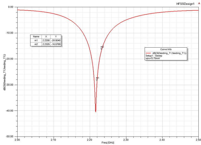
Fig. 1.18: Reflection coefficient for the case when two grounds are connected.
