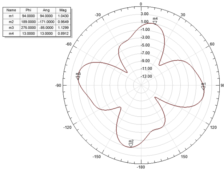
Fig. A.44: 2-D gain plot for \theta = 90 degree of four S-band antennas with 12 additional microstrip dipoles.
