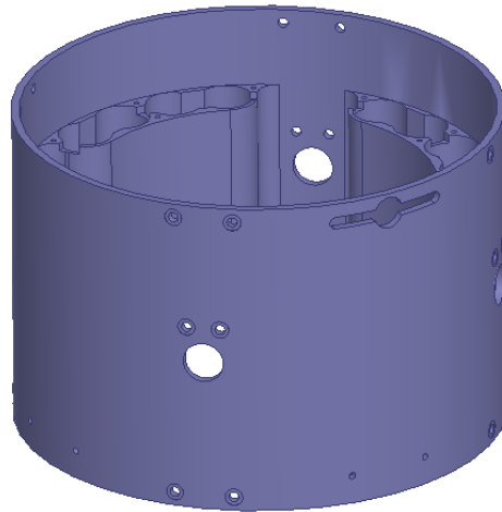
Fig. 1.3: Core of the sub-payload to be placed under the multi-layer substrate.
