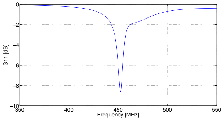
Fig. 2.16: Reflection coefficient of bottom slot for simulation model-I.
