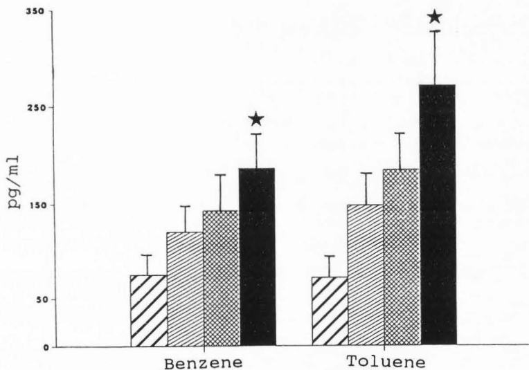
Fig. VII-1. Effect of 4 — weeks benzene and toluene exposures via drinking water on concentrations of plasma ACTH in mice ( \square , control; \text{▨} , 31 mg/L for benzene and 17 mg/L for toluene; \text{▩} , 166 mg/L for benzene and 80 mg/L for toluene; \blacksquare , 790 mg/L for benzene and 405 mg/L for toluene). Stars (*) denote a significant effect ( p < 0.05 ) relative to control. Values represent mean \pm SE ( n=5 ).
