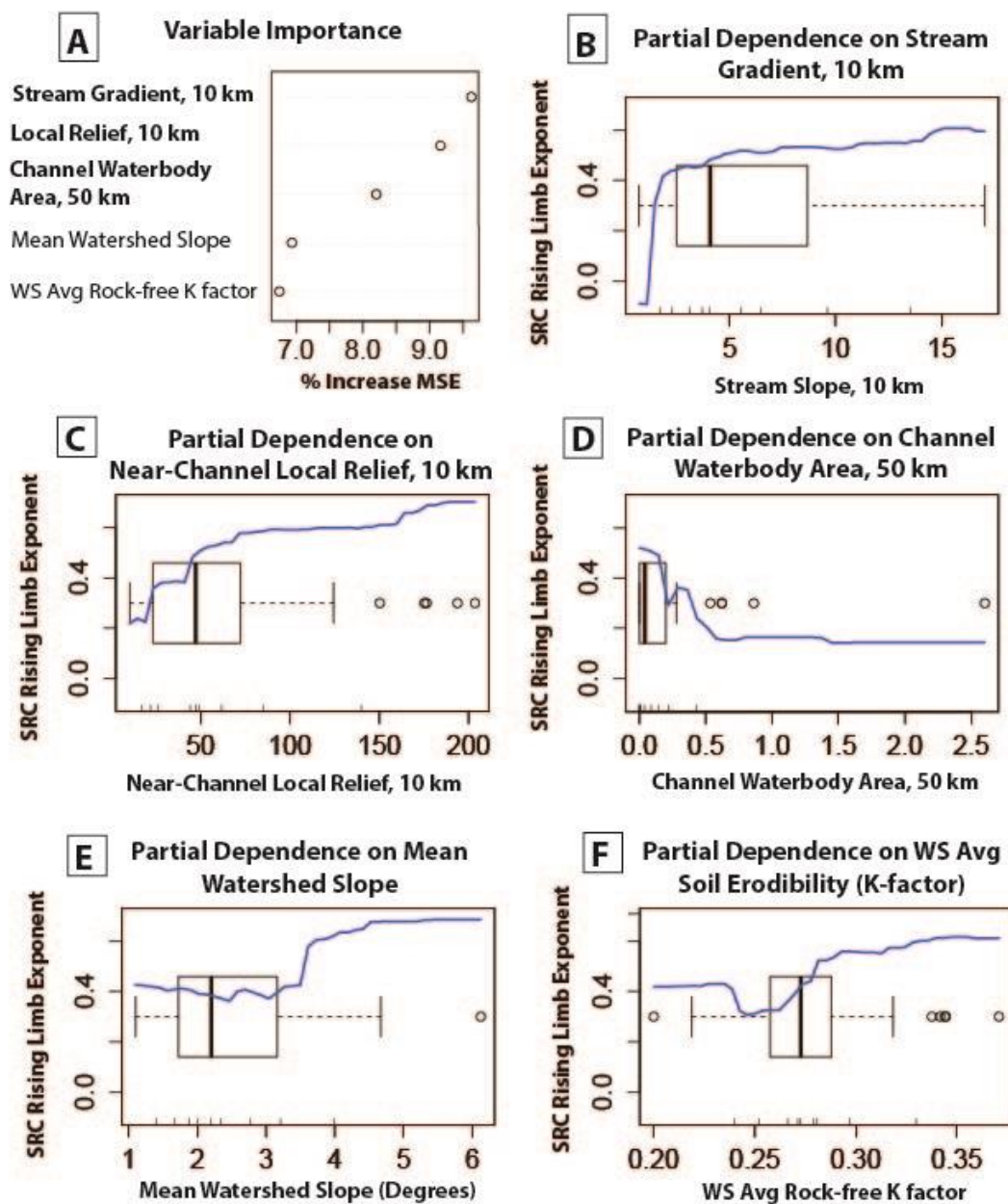
Figure 9. Results from Random Forest regression model for SRC rising limb exponent. A. Variable importance plot. X-axis shows the percent increase in model mean-square-error when values for the variable in question are permuted. Variables are ranked in terms of importance, with most important variable at the top. Near-channel metrics shown in bold, watershed-average metrics shown in regular font. B – F. Partial dependence plots showing estimated value of the SRC rising limb exponent given variations over the range of the selected predictor variable. Also shown on graphs are box-and-whisker plots showing distribution of values for each predictor variable.
