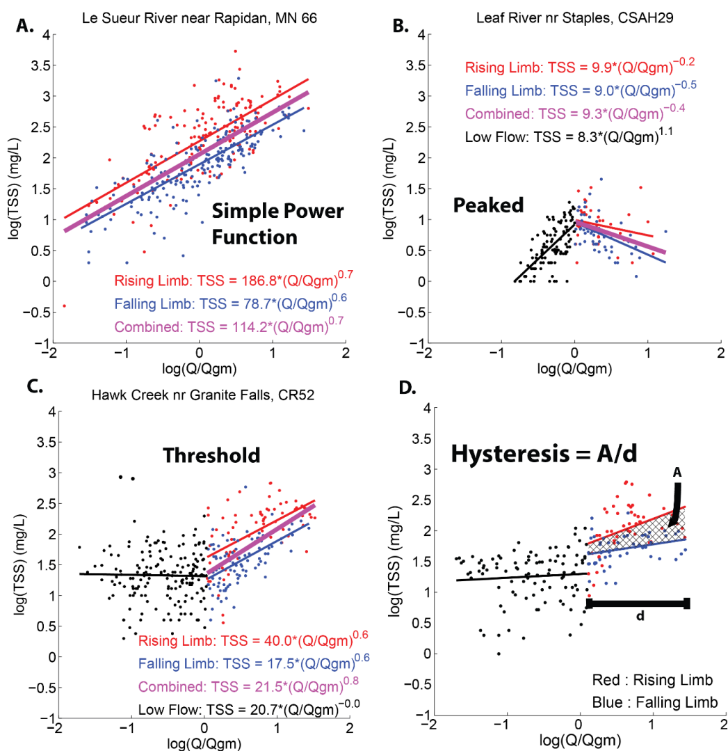
Figure 3. A – C. Representative Q-TSS relationships, showing the three broad categories of relationships observed. D. Explanation of computation of hysteresis metric.
