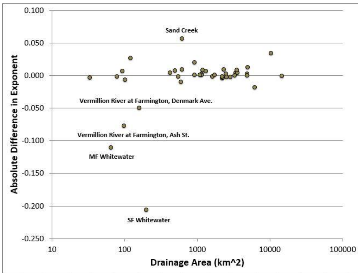
Figure B.1. Absolute difference in rating curve exponents for SRCs created using mean daily and instantaneous flow data.
