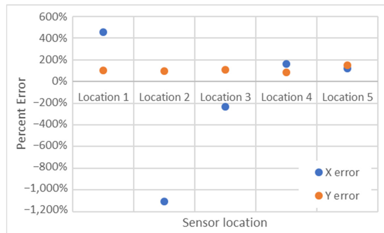
Figure 5. Grain bin strain error comparison.
