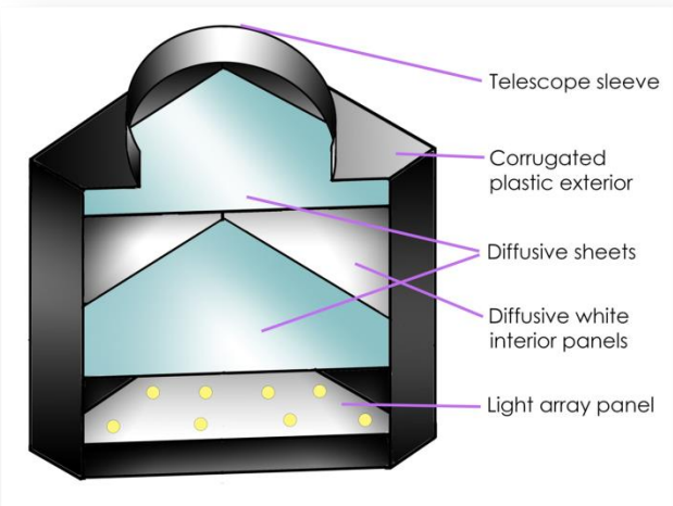
Figure 3: Schematic of the flat field box.
