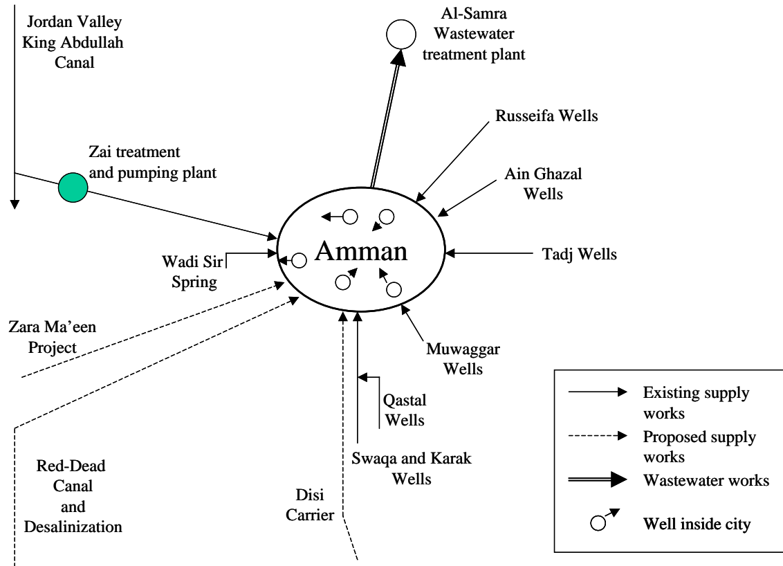
Figure 2. Schematic of existing and proposed main water supply and wastewater works for Amman
