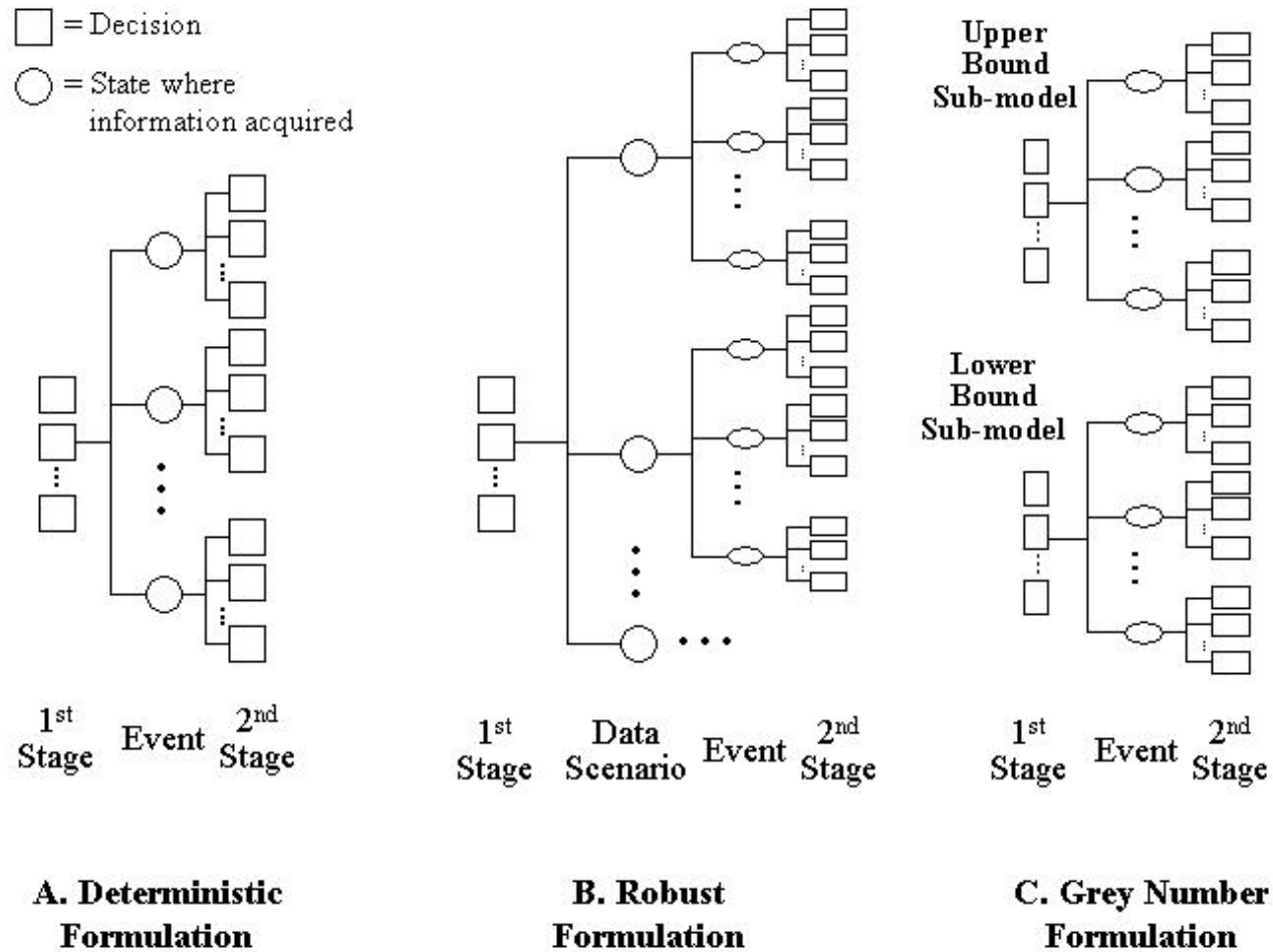
Figure 1. Decision trees for stochastic programs with recourse
