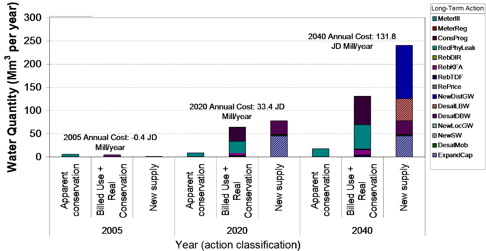
Figure 4. Capacity expansion and expected costs to cope with shortages over time
