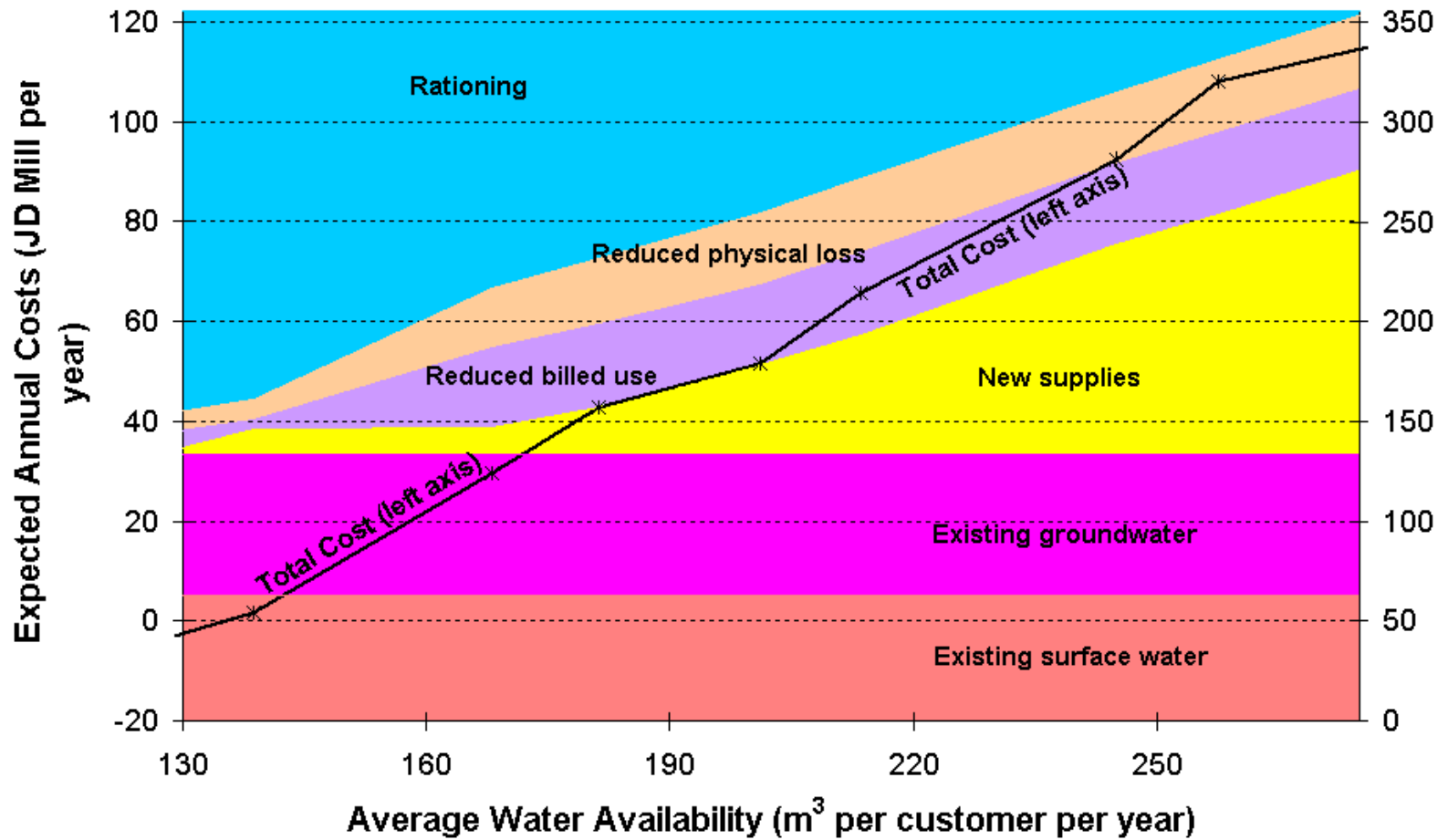
Figure 5. Costs associated with increasing water availability to customers
