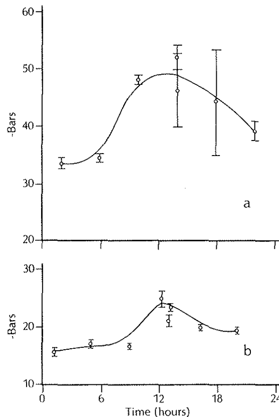
Figure 6. Water plant potential of the creosotebush plant; a is for August 20, 1974; b is for November 1, 1974.
