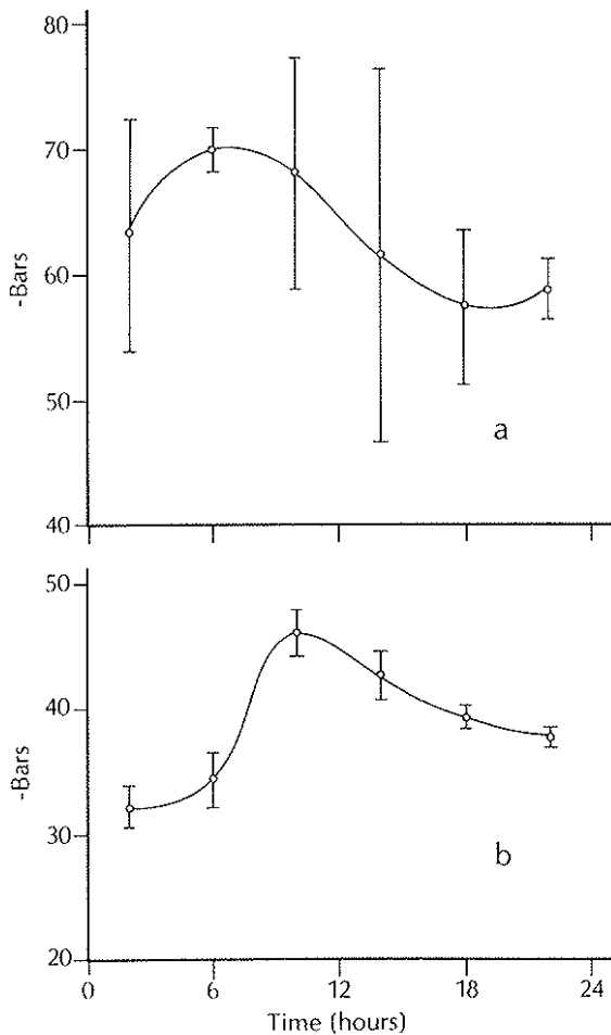
Figure 4. Water plant potential of the creosotebush plant; \bar{x} = one standard deviation; a is for June 13, 1974; b is for July 17, 1974.
