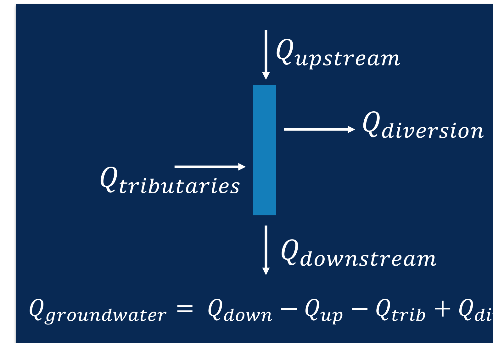
Figure 2: Flow measurement
