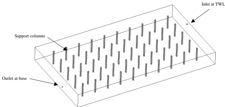
Figure 1. Schematic layout of the proposed service reservoir.
