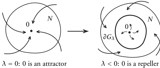
FIGURE 4.1. Attractor-bifurcation
