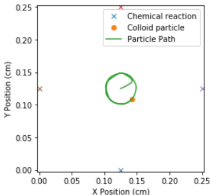
Figure 6: Motion in a circular pattern created using a chemical gradient. The strengths of the four sources of chemical reaction are varied with time to produce the desired path.
