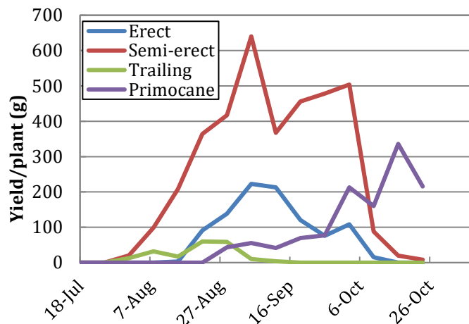
Figure 1. Time course of each growth type in 2011. The best performing cultivar from each type is shown. They are Navaho, Lochness, Metolius, and Prime Jan.
