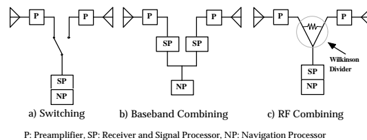
Fig.7 Configuration of GPS Receiver and Antennas.
