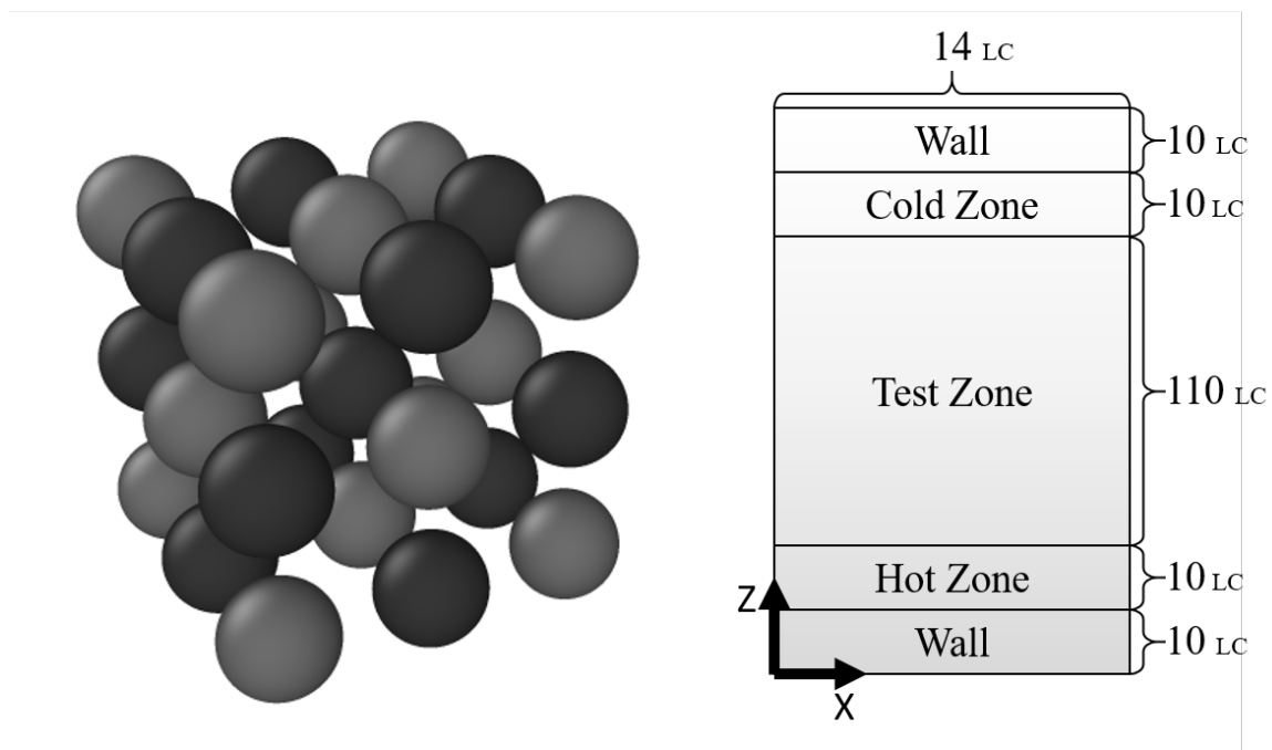
Figure 3: Crystal lattice (left) and model diagram (right). The model diagram shows cross section of rectangular prism 14 x 14 x 150 lattice constants. (LC = 4.698Å)
