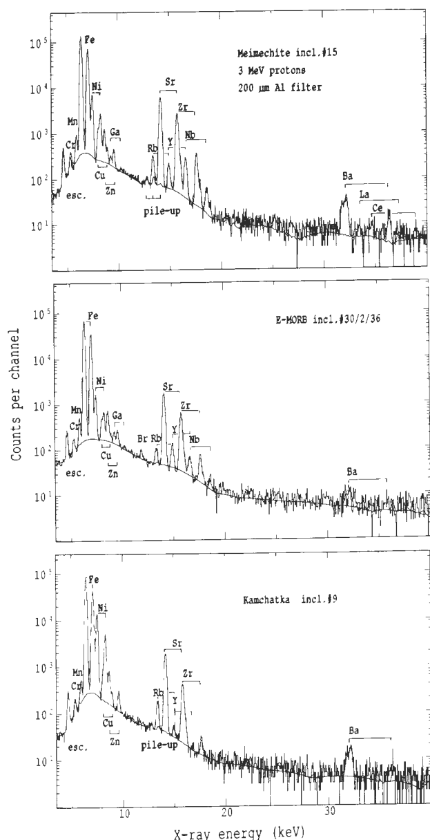
Figure 4. Spectra from melt inclusions in olivine from ultramafic rocks from different tectonic settings: continental lithosphere (top), mid-ocean rifts (middle) and subducted zone (bottom). The trace elements of interest are Rb, Sr, Y, Nb, Zr, Ba which are completely incompatible with olivine. The Ni observed in the spectrum is due to the olivine and is used to estimate the olivine contribution to the spectrum. The ratios of these elements to the Y content however should be unaffected and as can be seen vary widely with the different tectonic setting.
