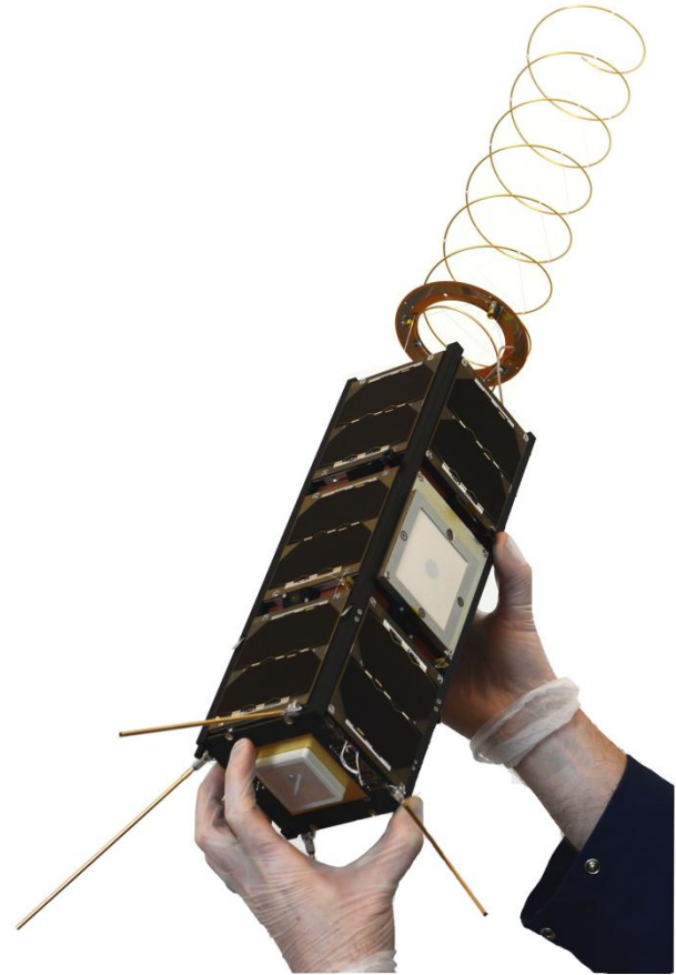
Figure 6 : The GOMX-3 satellite
