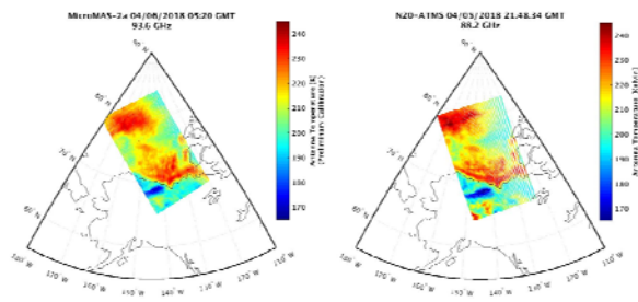
Figure 2: MicroMAS-2a on-orbit data (left) compared to NOAA-20 ATMS data (right) observed approximately seven hours earlier.
