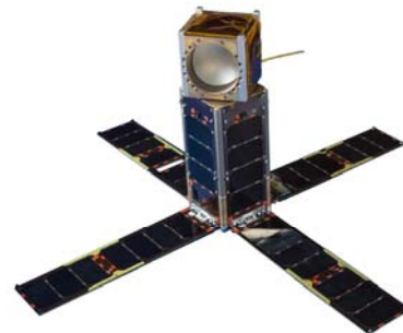
Figure 1: The MicroMAS-2a satellite is 4.5 kg and 34 x 10 x 10 cm 3
