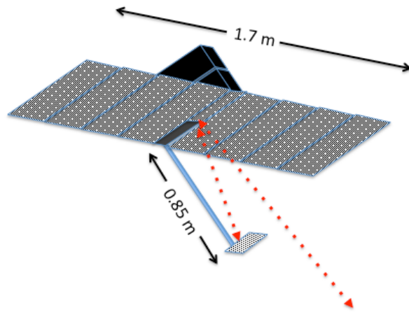
Figure 6: Ka-Band SAR concept shown in deployed configuration. Design stows into a 12U volume.
