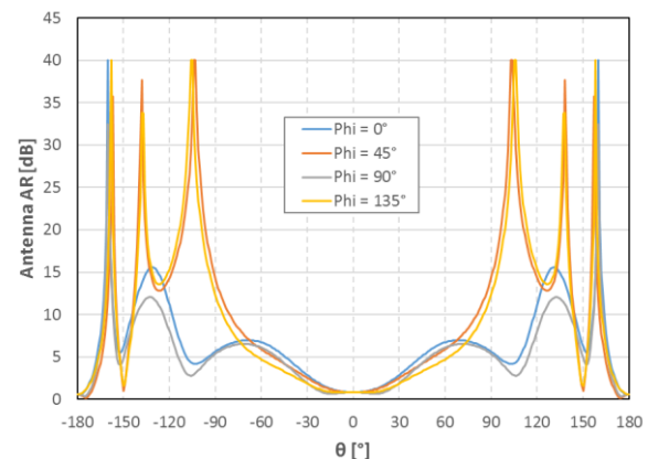
Figure 14 : Integrated Antenna AR Performances at 1700MHz
