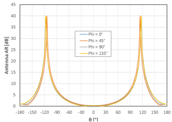
Figure 12 : Integrated Antenna AR Performances at 400MHz
