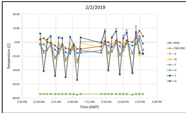
Figure 10: On-orbit Temperature Data, First Week Mode, February 2, 2019
