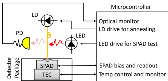
Figure 1: Concept of the in-orbit laser annealing. Laser diode (LD) produces a high-power optical beam used to anneal the SPADs. LD output is guided to the active area of the SPAD through an optical fibre. A light emitting diode (LED) is a reference light source to monitor detectors’ photon detection efficiency. Photodiode (PD) monitors the power illuminated to the SPAD. TEC is an integrated thermoelectric cooler with the SPAD.
