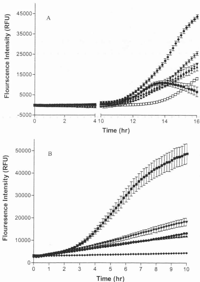
Figure 5-4. Effect of various activators and inhibitors on maturation of B. linens BL2 protease. Panel A: For heterogeneous protease activation experiments, 29.1 µg/ml B. linens BL2 protease is used. Proper heterogeneous protease activity controls are subtracted. In the case of B. linens BL2 protease, total 58.2 µg/ml BL2 protease is used and the protease activity above 29.1 µg/ml protease control is represented. ▲ subtilisin Carsberg (1 mU/ml); ■ subtilisin Carsberg (0.1 mU/ml); ◆ Bovine plasmin (1 mU/ml); ● Cathepsin D (10 mU/ml); □ Chymosin (1 Milk Clotting Unit/ml); ■ B. linens BL2 protease (29.1 µg/ml); Panel B: For each of inhibitor experiment, 29.1 µg/ml B. linens BL2 protease is used. ◆ EDTA (1 mM); ▲ p -Hydroxy mercuribenzoate (PCMB) (1 mM); ▼ Iodoacetic acid (1 mM); ● Mn 2+ (1 mM); ■ B. linens BL2 protease control.
