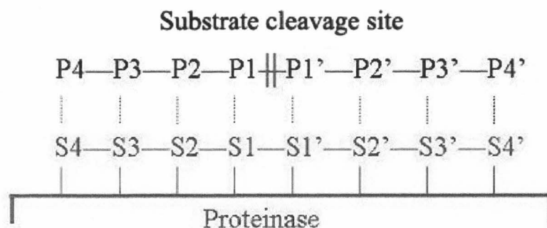
Figure 2-3. Number system to describe the specificity of a proteinase (75).
