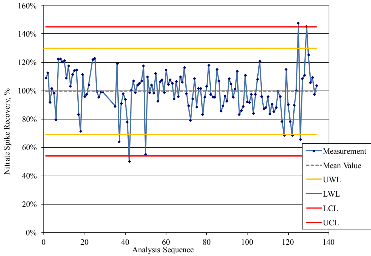
Nitrate Control Charts – Spike Recovery, %
