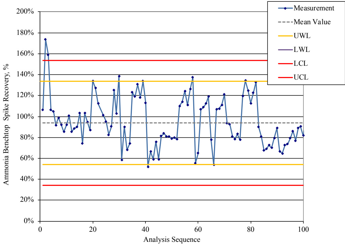
Ammonia Bench Top Analysis Control Charts – Spike Recovery, %
