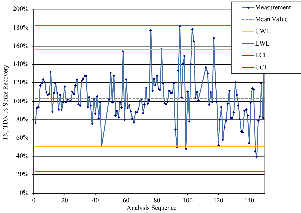
TN, TDN Control Charts - % Spike Recovery
