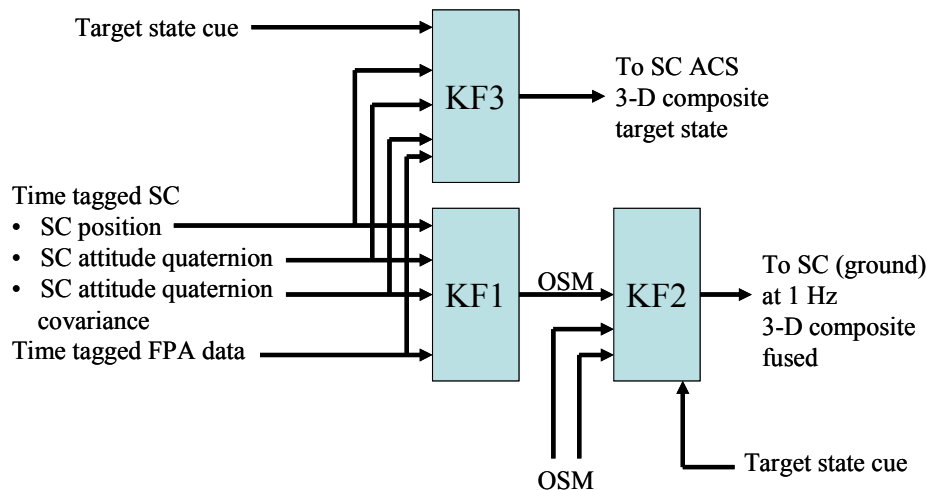
Fig. 6. Filter fusion architecture per satellite
