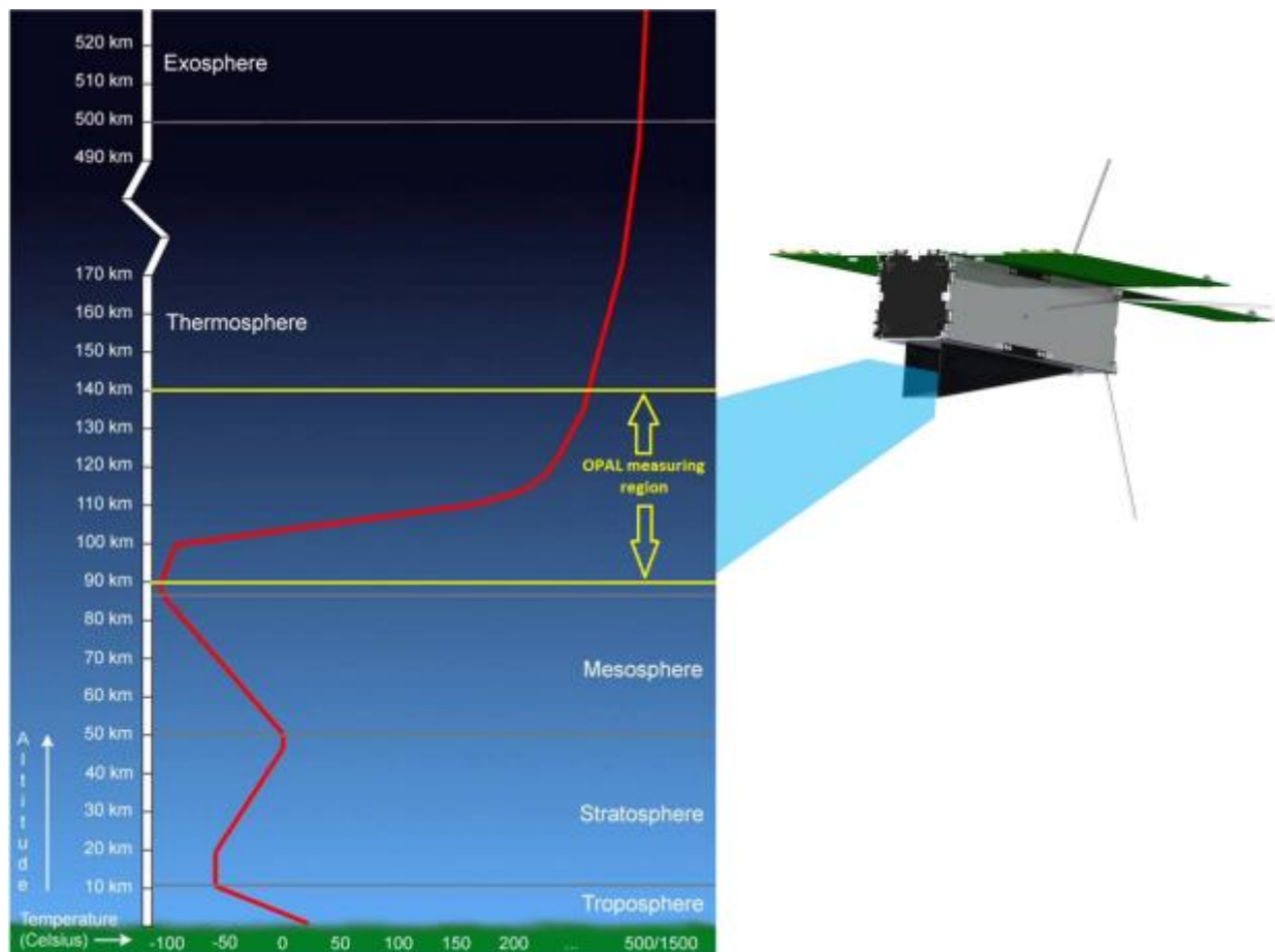
Figure 1: The OPAL CubeSat shown with its intended field of view (FOV) in the lower thermosphere. [2,6]
