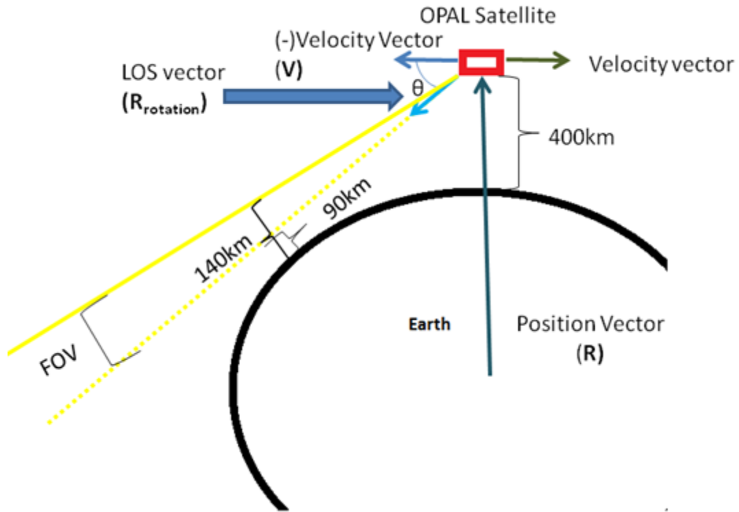
Figure 4: Visual interpretation for the use of the Rodrigues' rotation formula, and its use in the LOS and FOV.
