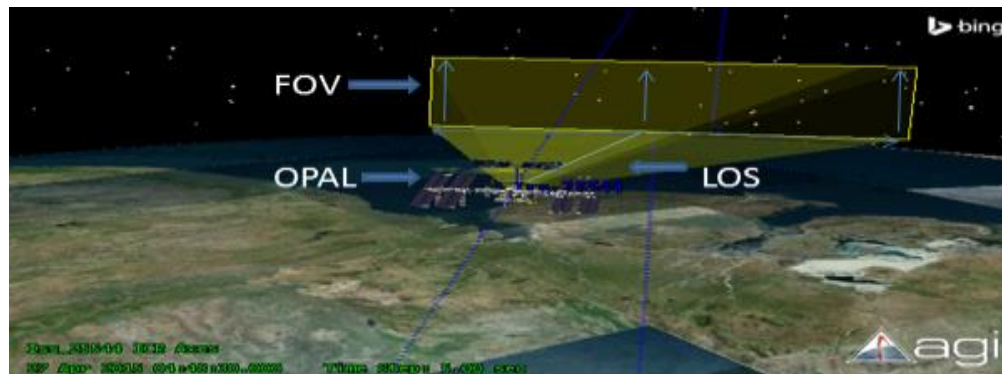
Figure 6: Model of the OPAL (3D-modeled with the ISS) orbit (blue), FOV (yellow), and light blue line denoting the originally calculated LOS with the light blue arrows showing where the line of sight needs to be included to the entire FOV to get a complete picture of the OPAL instrument's output.
