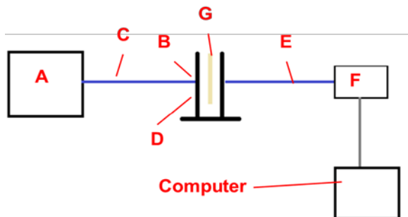
Fig. 1: Schematic of the experiment setup. The Deuterium light source (A) is connected to a fiber optic cable (C) which goes to a lens expander (B) attached to the sample holder (D). The sample (G) goes between the two posts of the sample holder. Another fiber optic cable (E) is attached to the opposite side of the sample holder, which goes to the Spectrometer (F). The spectrometer then hooks up to the computer where the data is imported into the Spectra Suit program.
