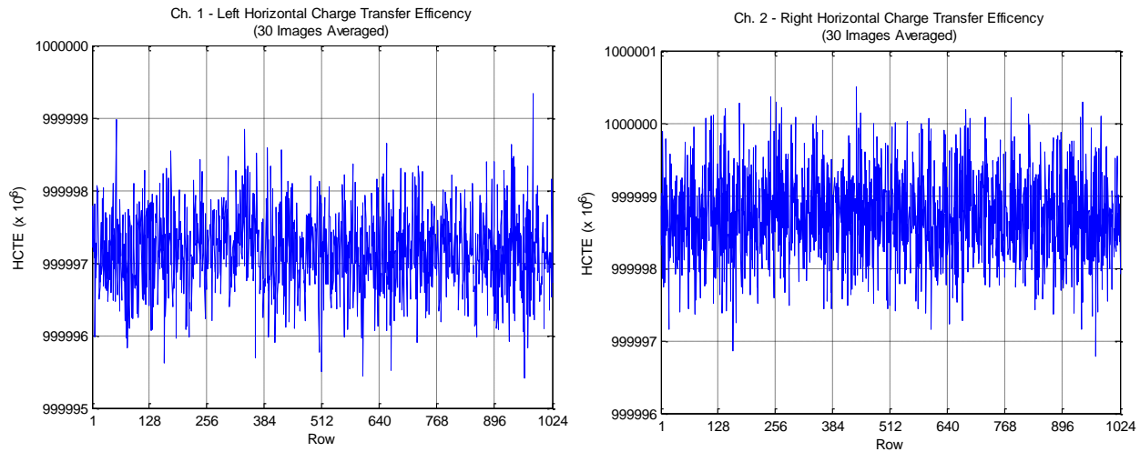
Figure 8. The HCTE of the left and right output taps of the CCD.
