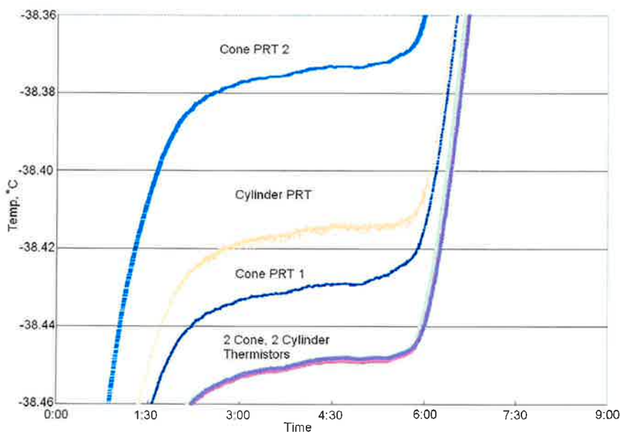
FIGURE 6. Readings from 3 PRTs and 4 thermistors in the CORSAIR blackbody vs. time with the blackbody controlled to a constant -38.4 °C.
