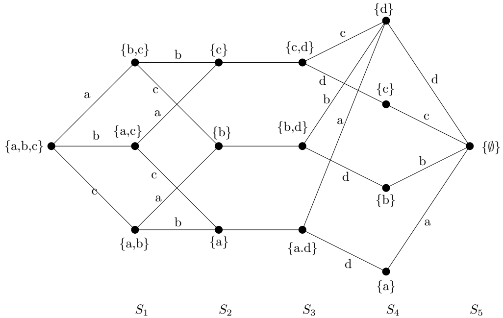
Fig. 3.7: Trellis representing an entering person.
