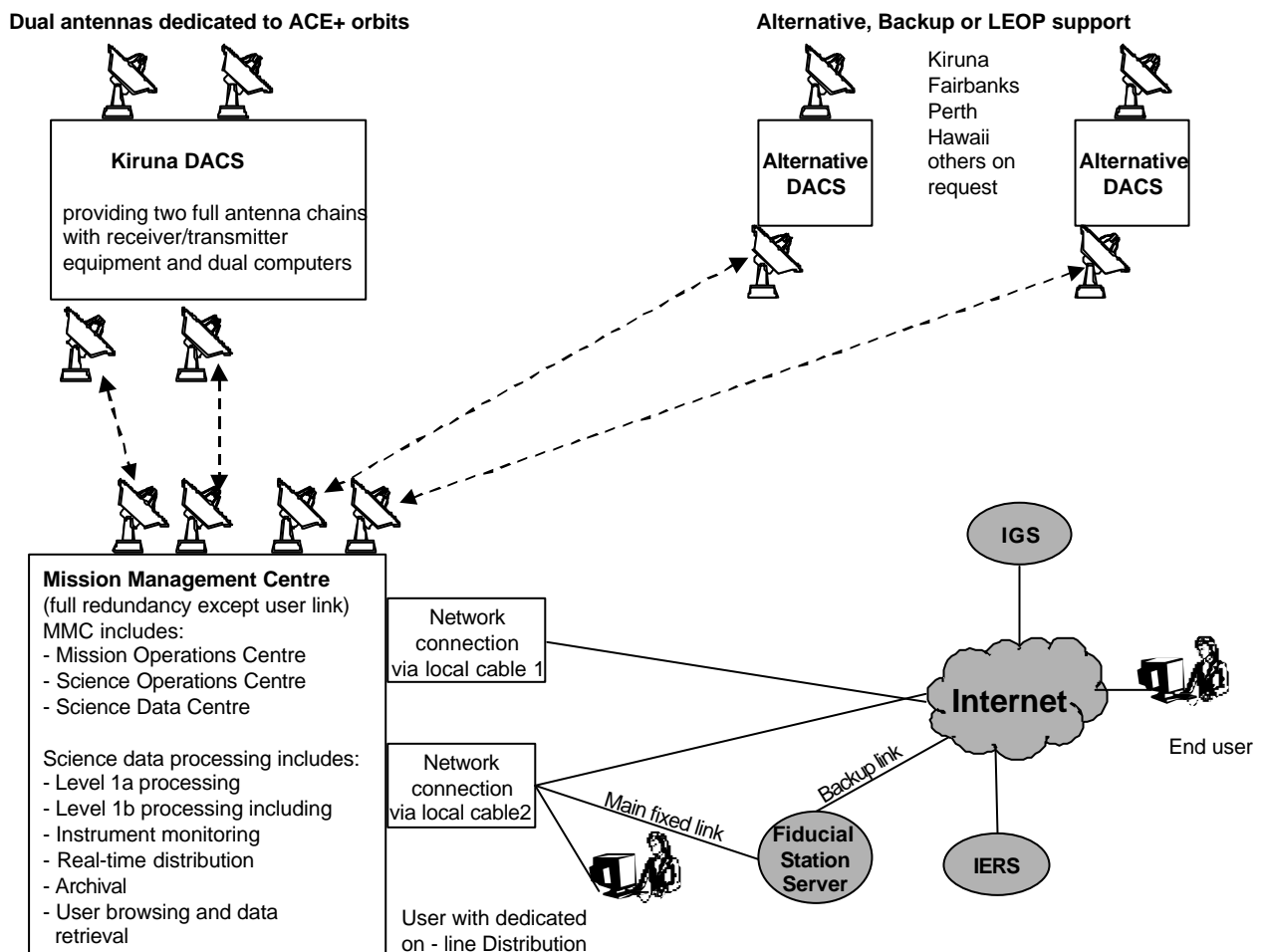
Figure 6: Overview of the ACE+ Ground Segment (Courtesy Terma)
