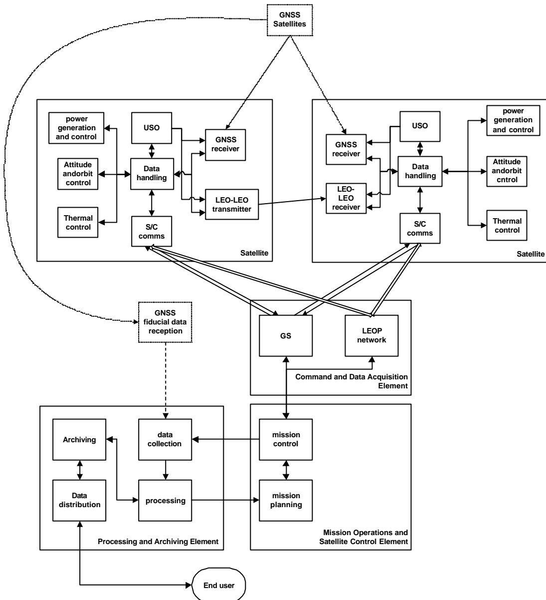
Figure 2: A Functional Architecture of the ACE+ Mission.
