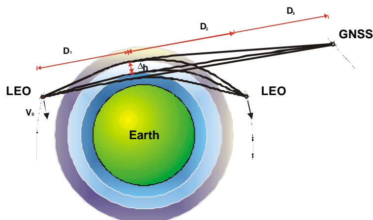
Figure 1: Outline of the Geometry for Radio Occultation Measurements Based on LEO-LEO and GNSS/GALILEO-LEO Observation Schemes
