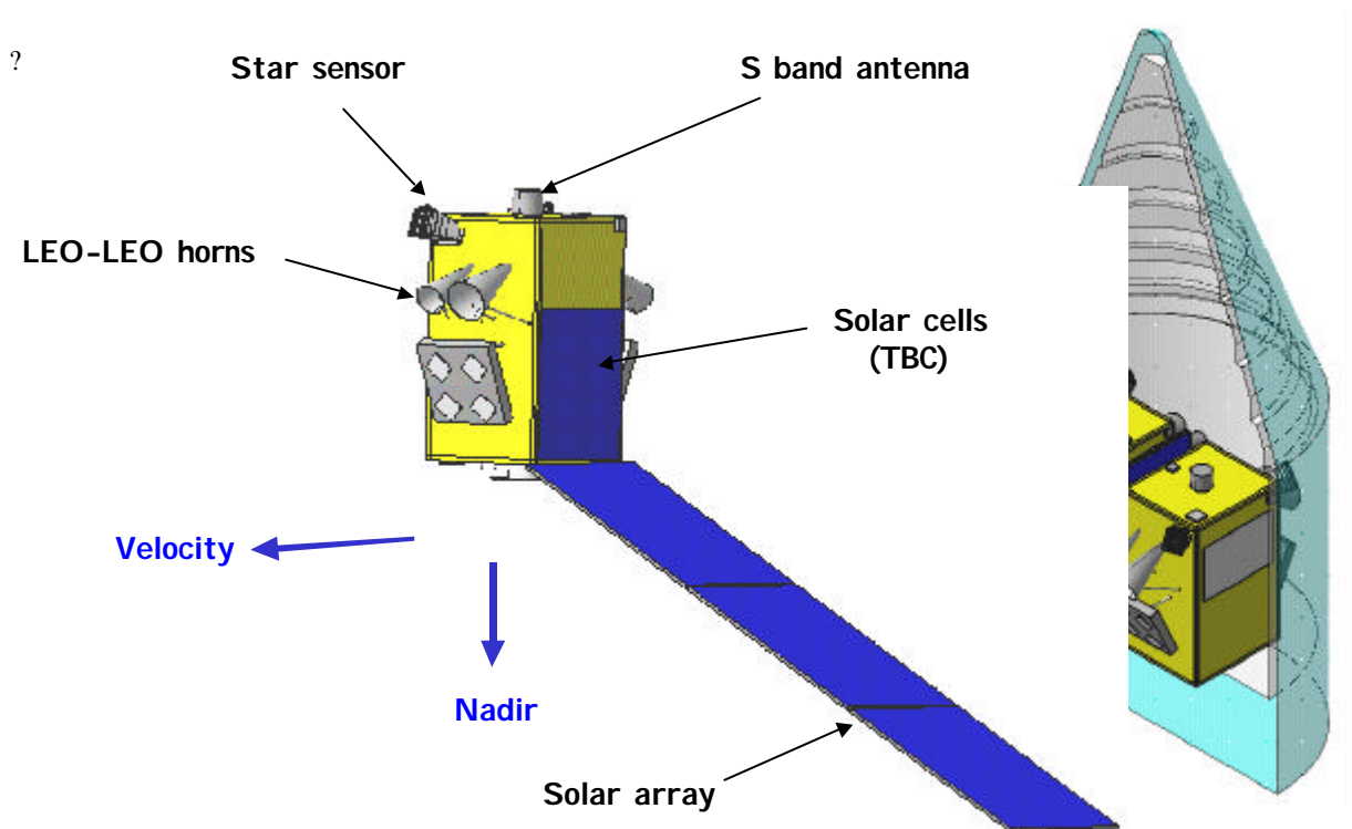
Figure 5: ACE+ Satellite Orbital Configuration and Two ACE+ Satellites under the Cosmos Fairing (Courtesy Astrium SAS)
