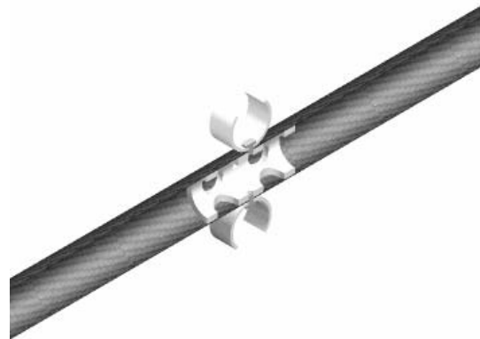
Figure 4: Deployed configuration with batten frame
