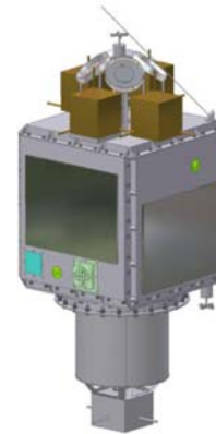
Figure 1: FalconSat-3 with EMC Boom and MPACS thruster mounted on bottom plane
